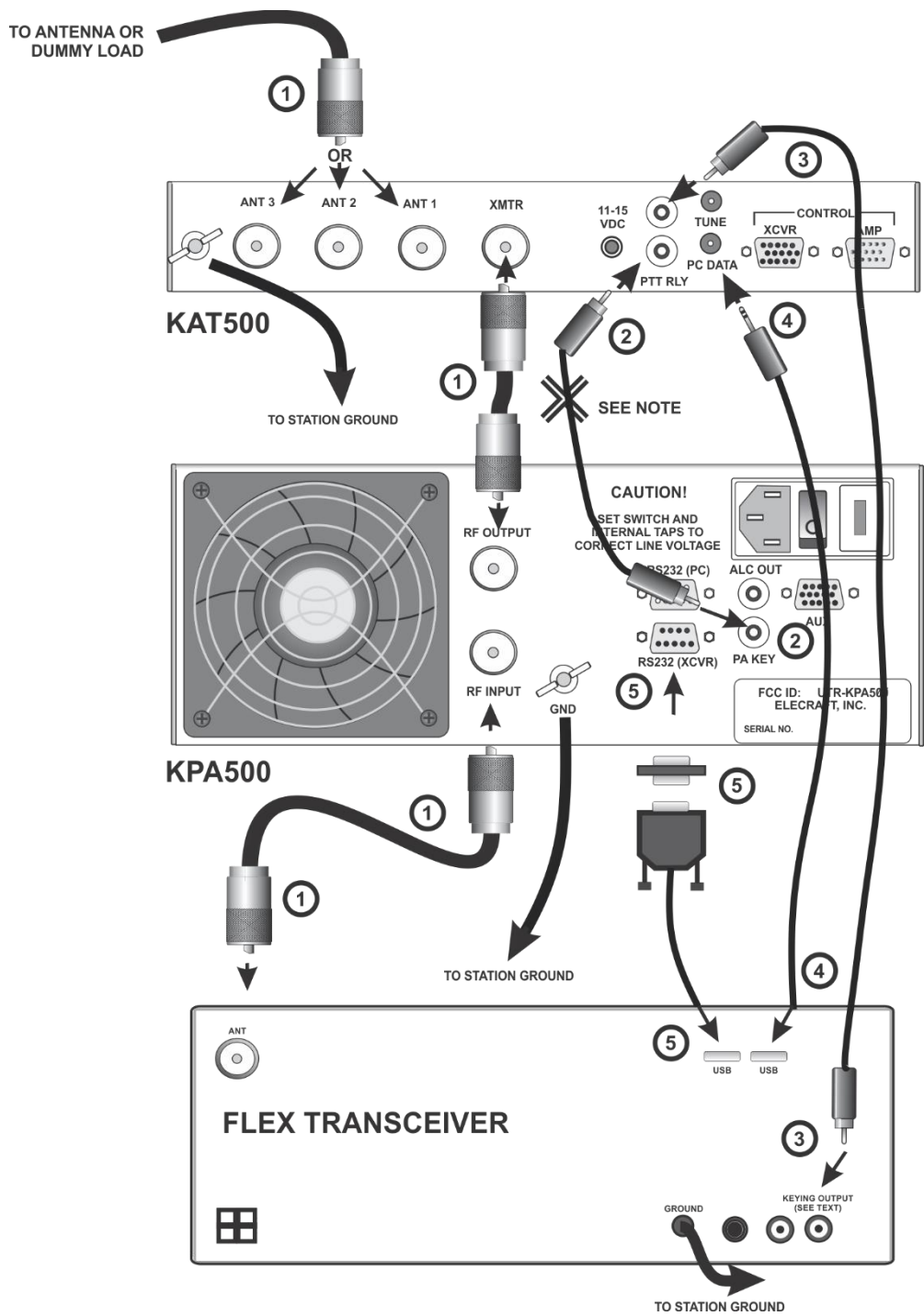
Figure 7. Cabling Diagram: Elecraft KAT50, KPA50 and Flex 6000-Series Transceiver
