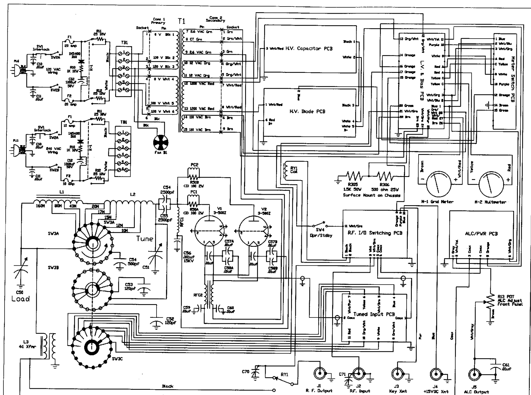
GRD TECHNOLOGIES, INC. Model HF-2000 Schematic Diagram Ray W. Connin January 13, 1995 Rev. 3r 06/22/99
