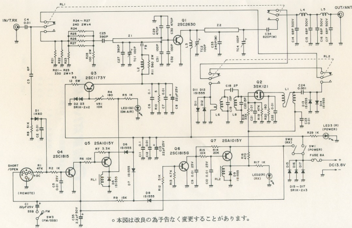
TOKYO HY-POWER HL-66V CIRCUIT DIAGRAM
