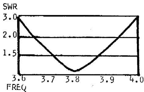
Figure 4: Typical SWR curves with antenna installed as an inverted Vee, with center 30 feet high and ends 10 feet above ground.
