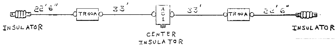
Figure 2: Permanent hookup. After passing through the eyebolt, wrap the wire around itself 5 times before soldering to the terminal.
