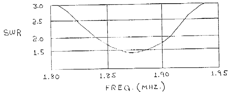
Figure 4: Typical SWR curves with antenna installed as an inverted Vee, with center 30 feet high and ends 10 feet above ground.
