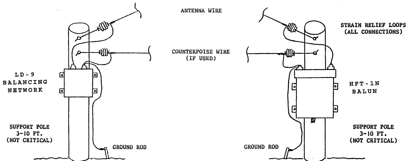
TYPICAL END-FED VEE INSTALLATION
