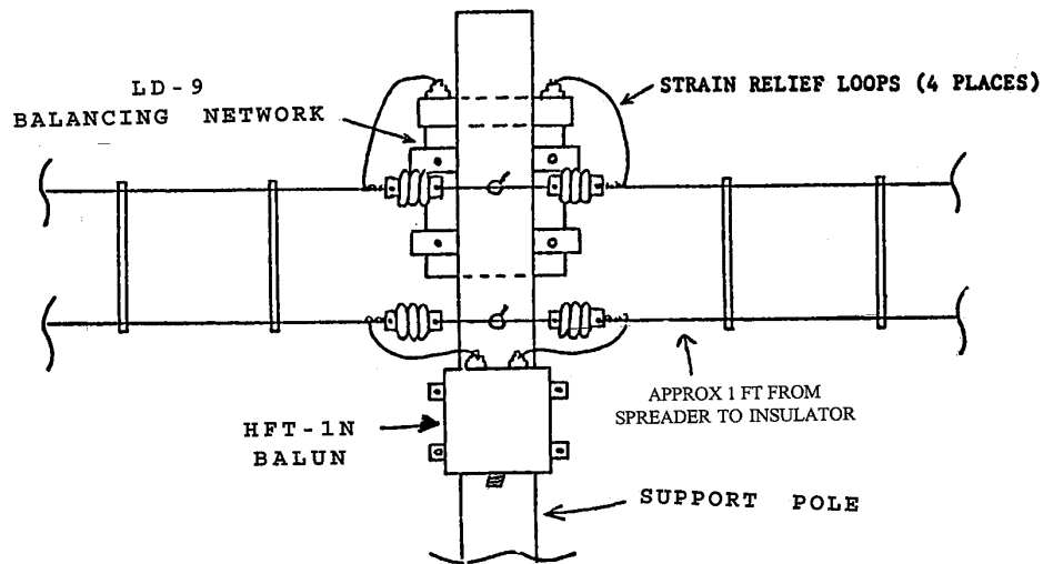
TYPICAL FOLDED DIPOLE INSTALLATION
