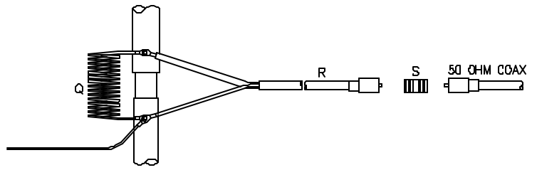
Feedline Detail
