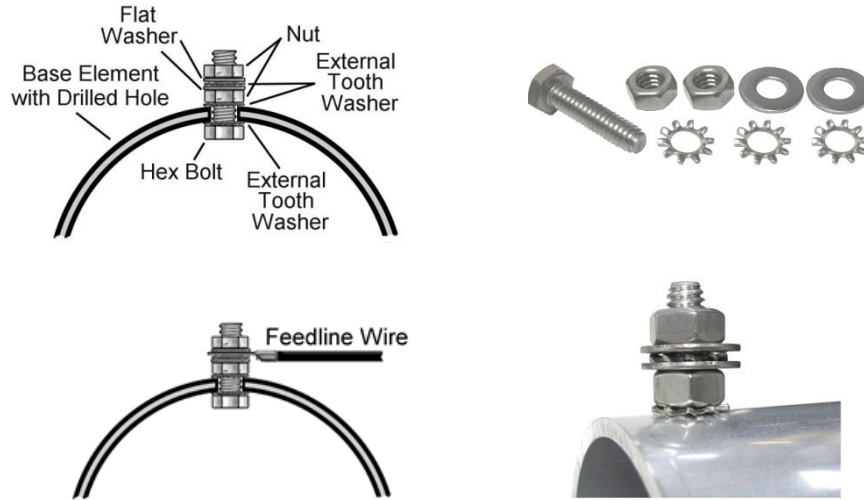
Views showing the Feedpoint hardware installed
