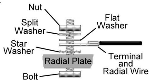
Radial Wire Hardware Installation
