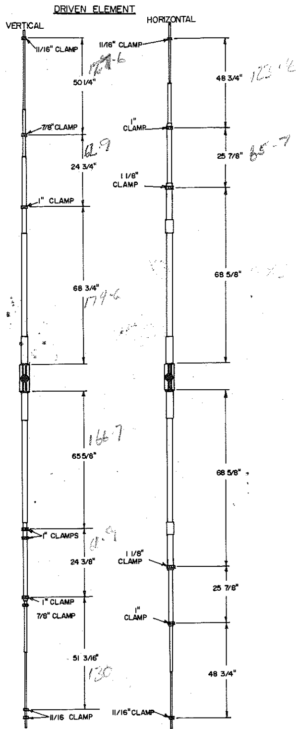
Figure 9. Driven Element Compression Clamp Assembly
