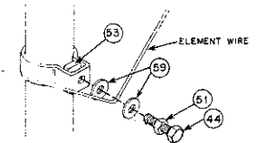
Detail "E"
