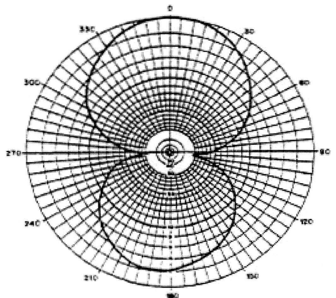
Radiation pattern with 1:1 Balun
