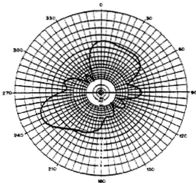
Radiation pattern without 1:1 Balun
