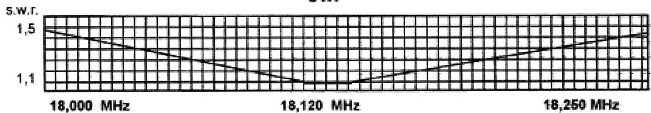
SWR
