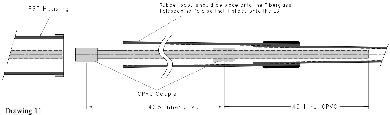
Fiberglass Telescoping Pole with Internal CPVC for 40/30m Diagram
