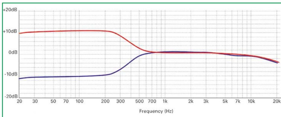
FIGURE 2: ParaPro EQ20 frequency response with the LF filter set to 300Hz +10dB (red) and -10dB (blue).
