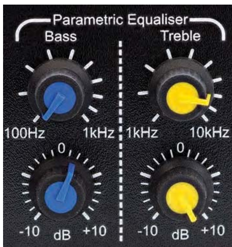
PHOTO 3: Close-up view of the filter control panel.
