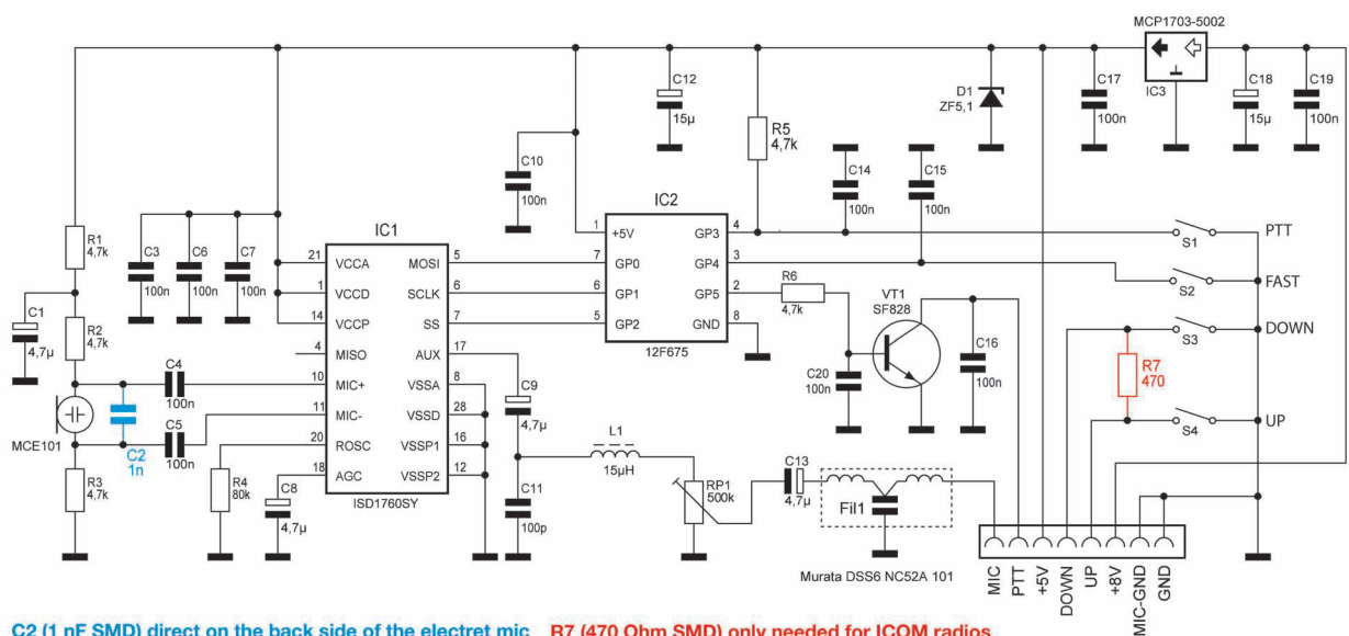
C2 (1 nF SMD) direct on the back side of the electret mic R7 (470 Ohm SMD) only needed for ICOM radios
