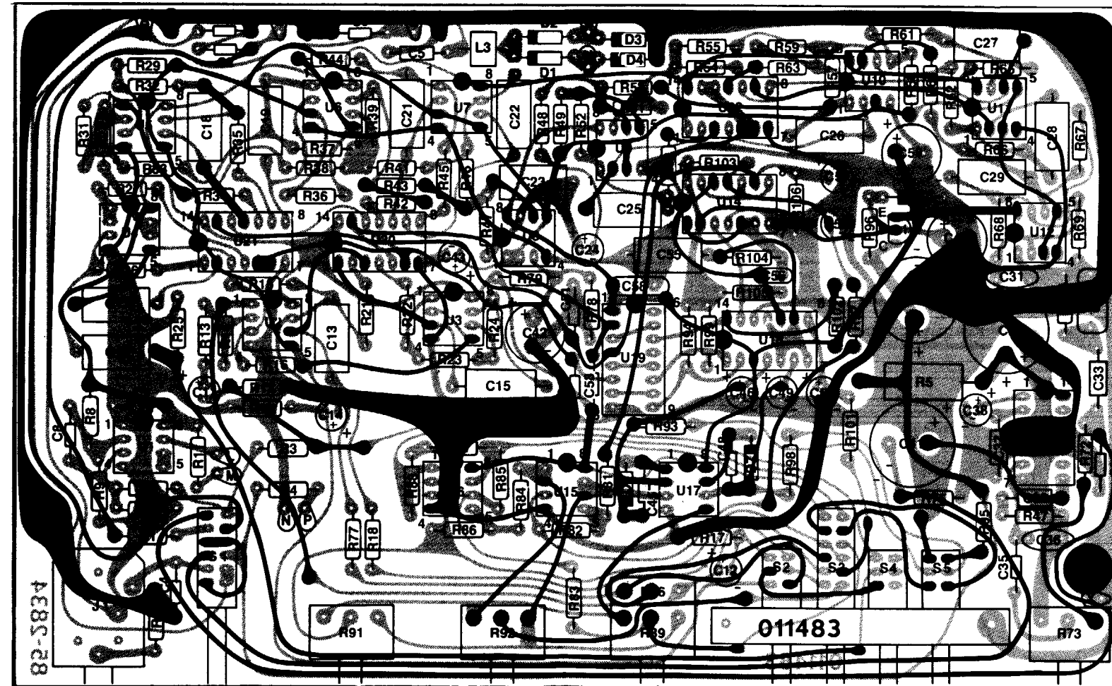
(Shown from the component side. The foil on the component side is shown in red.)
