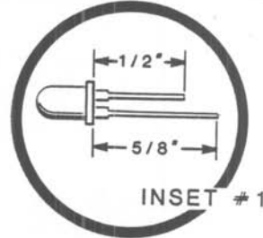
PICTORIAL 2-3
