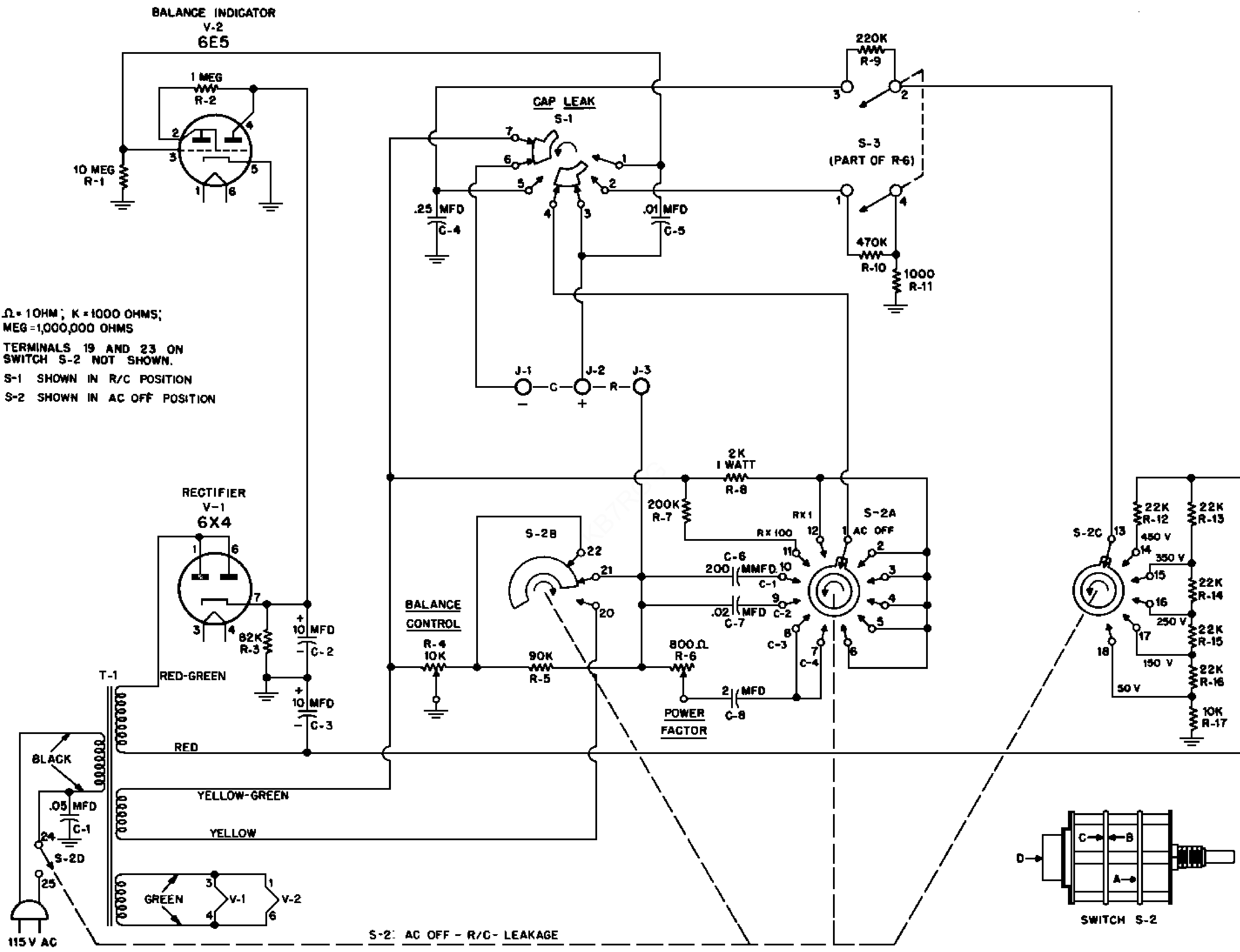
Resistor-Capacitor Tester
