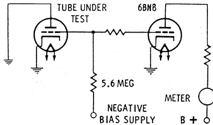
Figure 6—Grid Emission Test Circuit.
