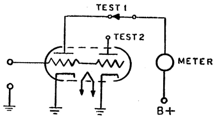
Figure 1—Each Section of Multisection Tube Tested Separately.
