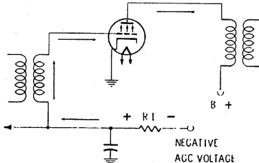
Figure 3—Typical I.F. Stage.
