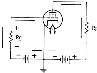
Figure 2—Negative Grid Current.
