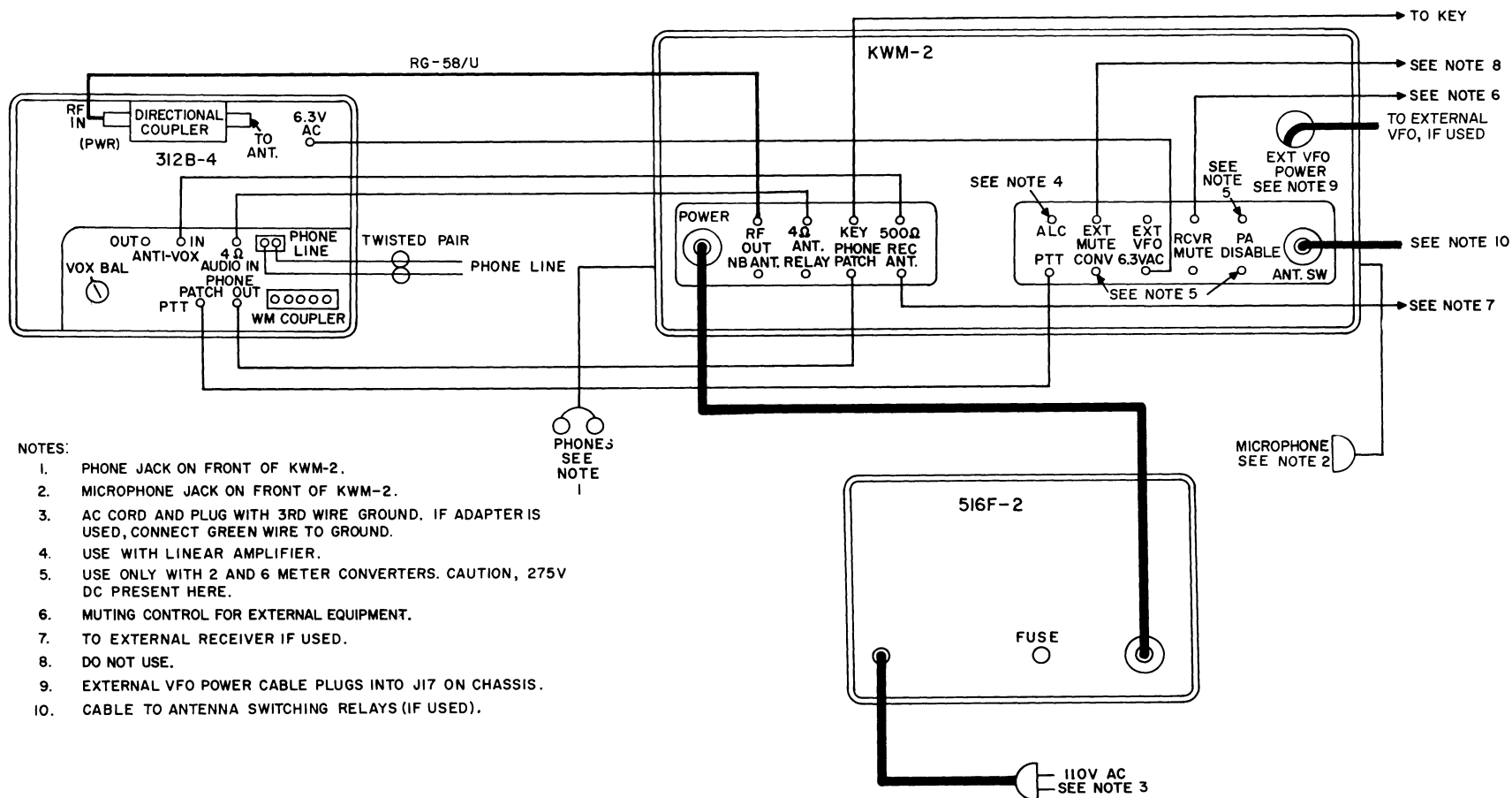
Figure 4. Interconnections, 312B-4 with KWM-2
