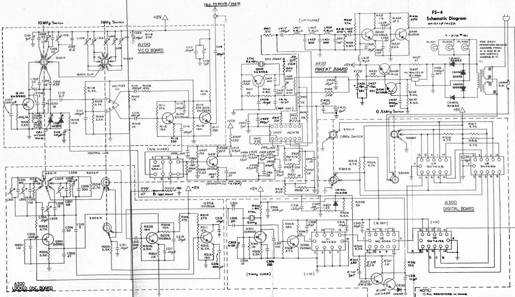
Figure 5-2. FS-4 Schematic Diagram
