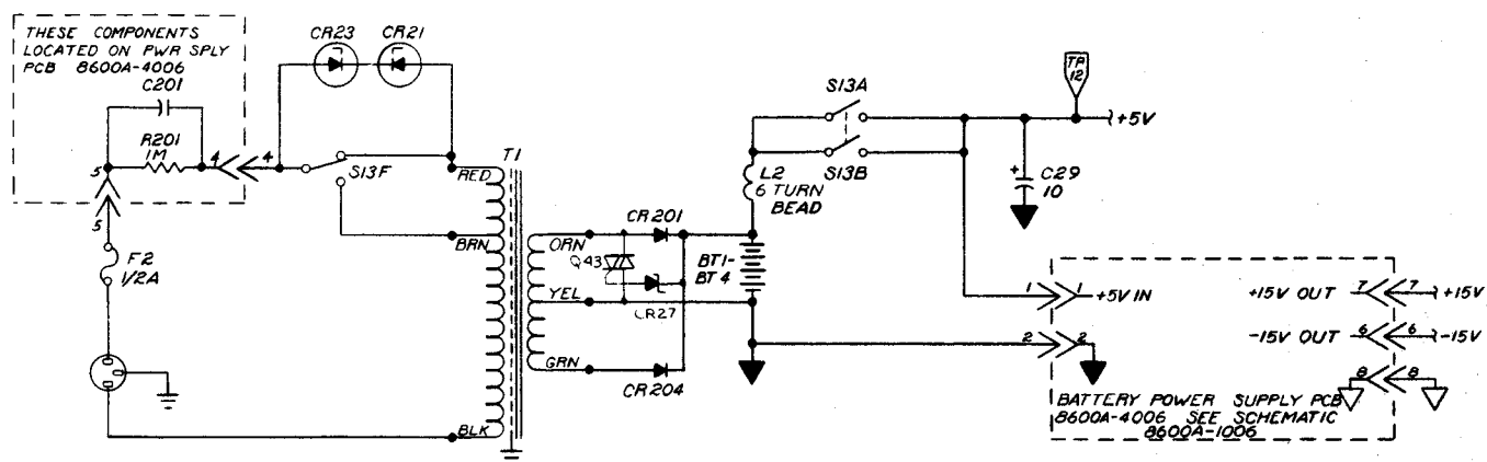
BATTERY POWER SUPPLY
