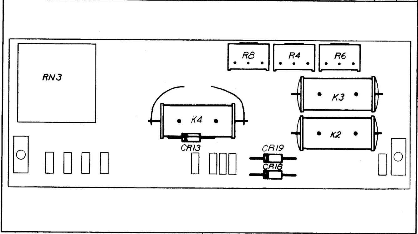
Figure 5-8. INPUT DIVIDER PCB ASSEMBLY
