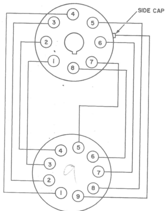
Fig. 2 (C) SJA-006 9-Pin Miniature Tube Adaptor
