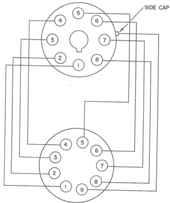
Fig. 1 (A) SJA-004 9-Pin Miniature Tube Adaptor
