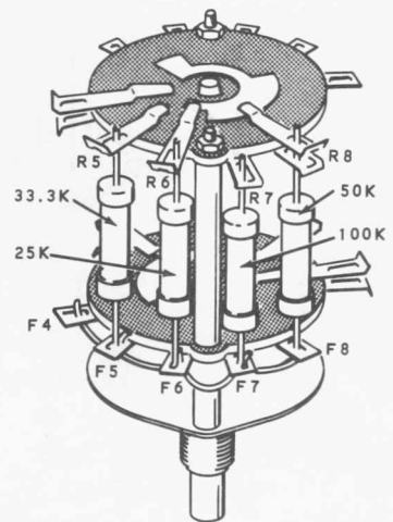
Detail 3B
