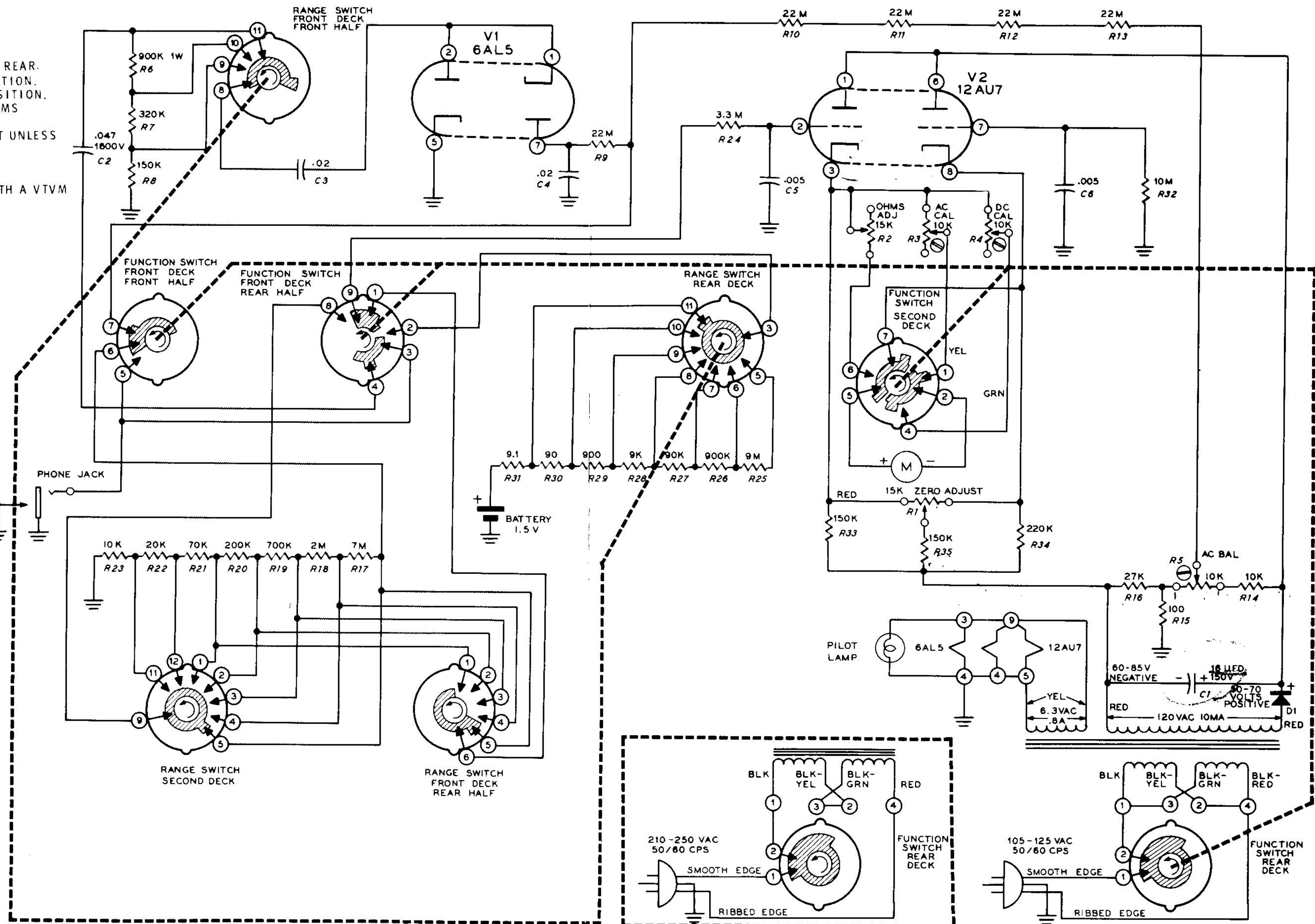
SCHEMATIC OF THE HEATHKIT® VTVM MODEL IM-18
