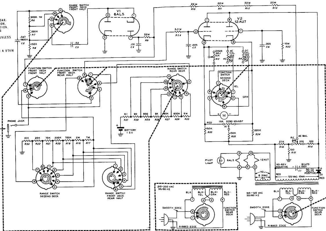
SCHEMATIC OF THE HEATHKIT® VTVM MODEL IM-18
