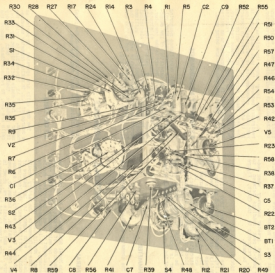
FIGURE 6.1 CHASSIS VIEW, MODEL 209A
