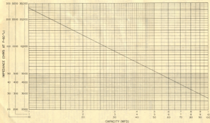
FIGURE 5.1 IMPEDANCE CHART
