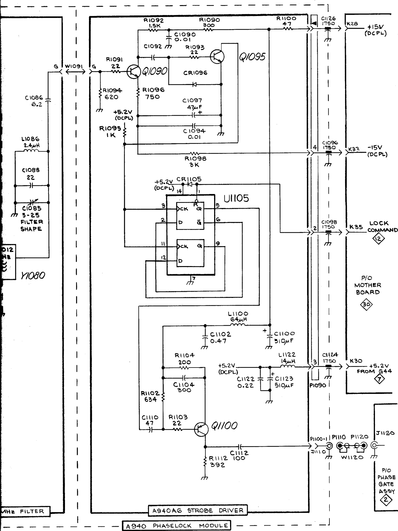
PL CONTROLLED OSCILLATOR, 16 MHz FILTER & STROBE DRIVER
