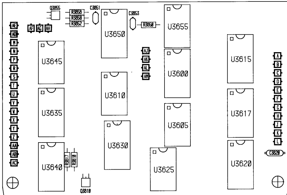
H-4969 DIGITAL STORAGE INTERFACE
