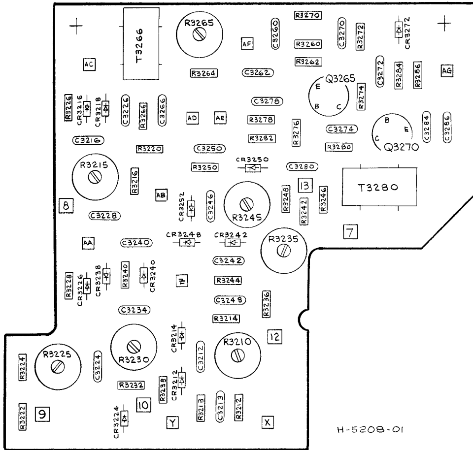
7L18 A3000A5 POST VARIABLE RESOLUTION AMPLIFIER
