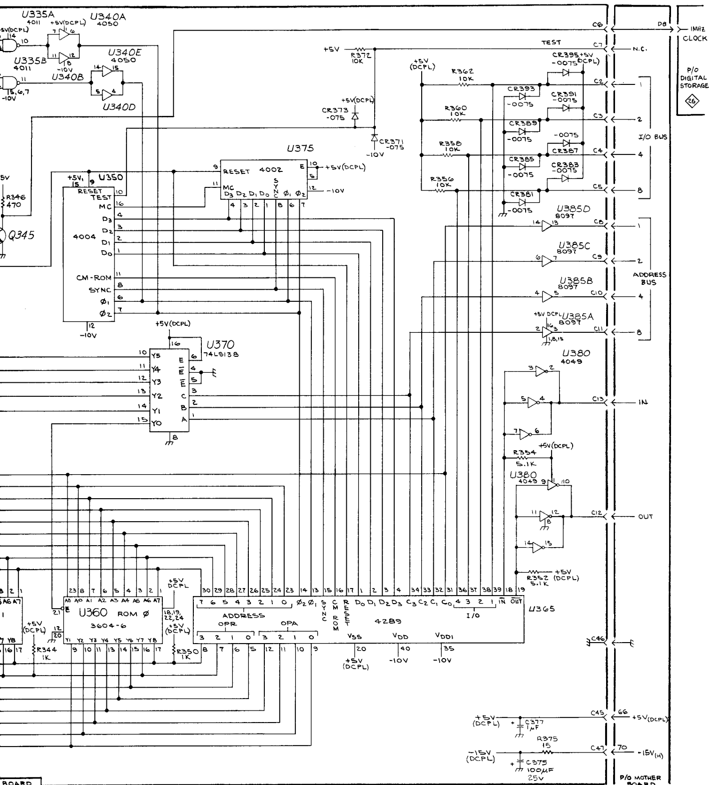
670-4505-00 MICROCOMPUTER 21
