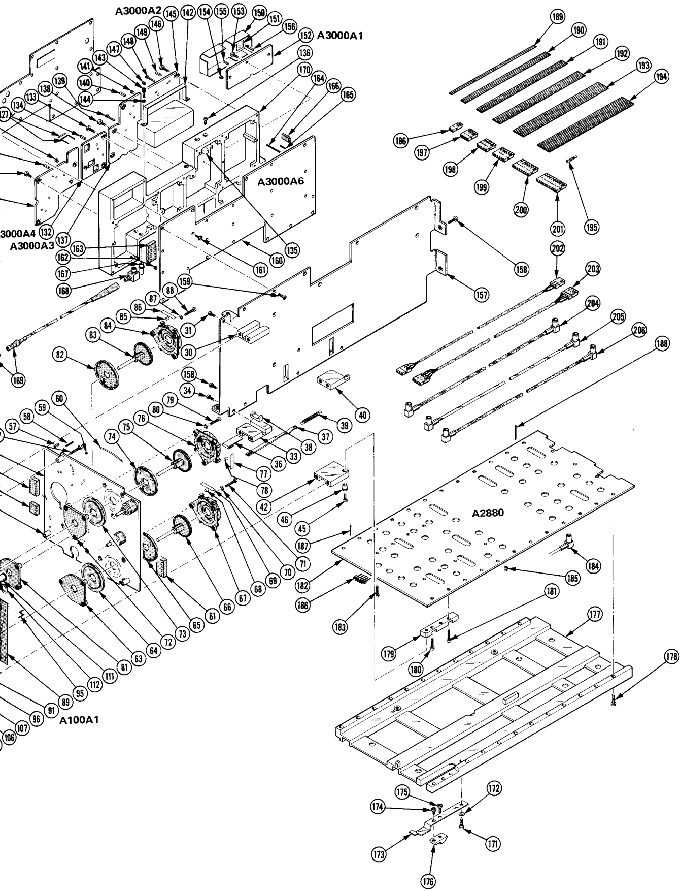
7L18 SPECTRUM ANALYZER
