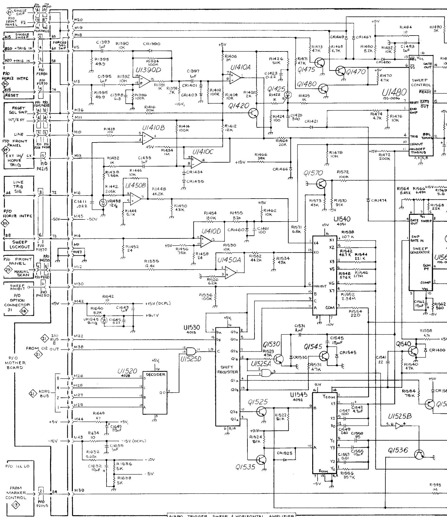
A1390 TRIGGER, SWEEP & HORIZONTAL AMPLIFIER
