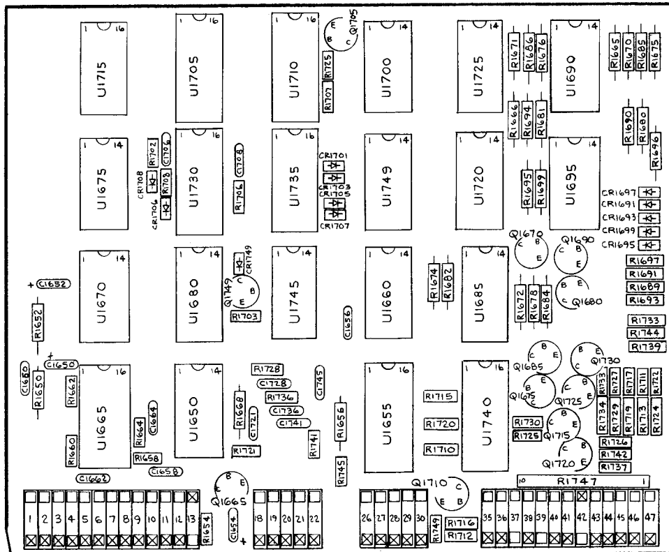
7L18 H-5023-01 A1650 CENTER FREQUENCY READOUT
