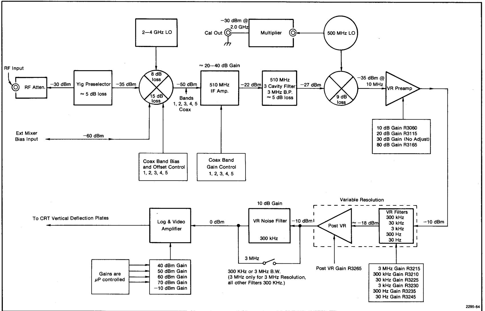
Fig. 4-52. Typical signal levels of the signal path through the 7L18.
