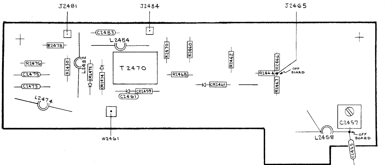
7L18 H-5320-01 A2360A2 2ND MIXER
