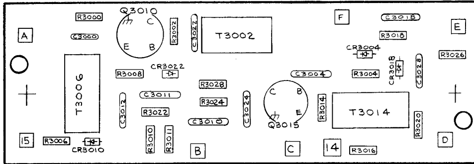
7L18 A3000A1 VARIABLE RESOLUTION INPUT H-5204-01
