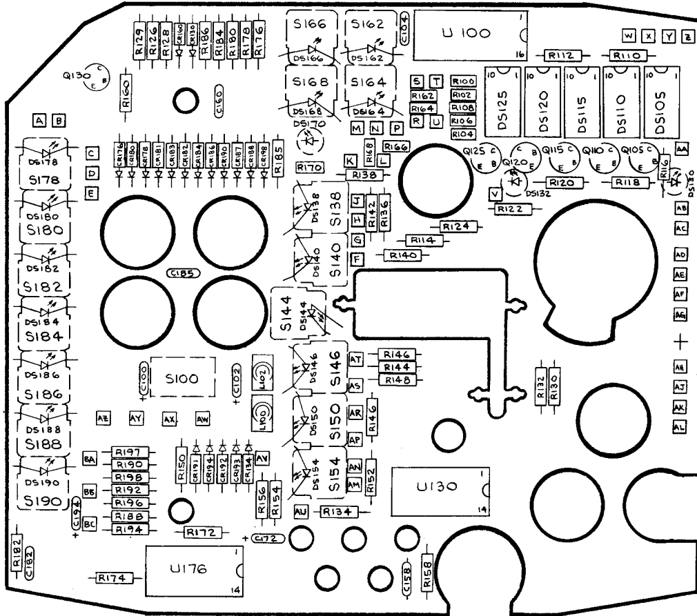
7L18 H-5025-01 A100A1 FRONT PANEL BOARD # 1
