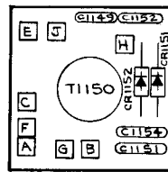
7L18 H-5045-01 A940A7A2 OFFSET OSCILLATOR RESONATOR
