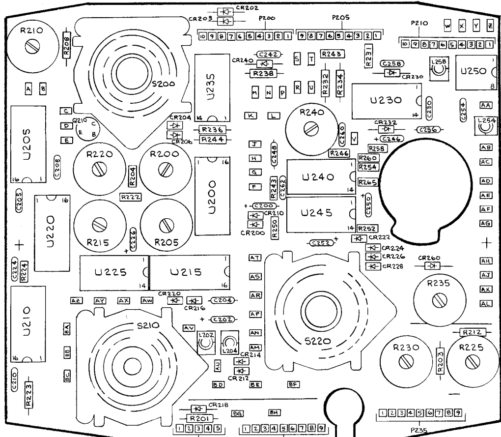
H-5030-01 P215 P220 7L18 A100A2 FRONT PANEL BOARD # 2
