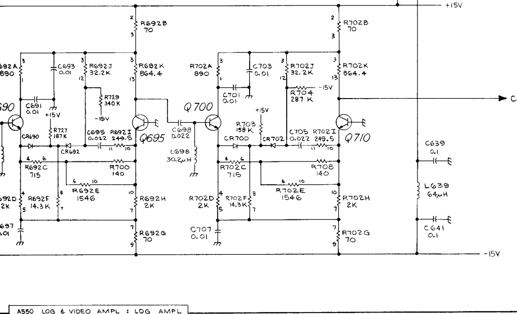
A550 LOG & VIDEO AMPL : LOG AMPL
