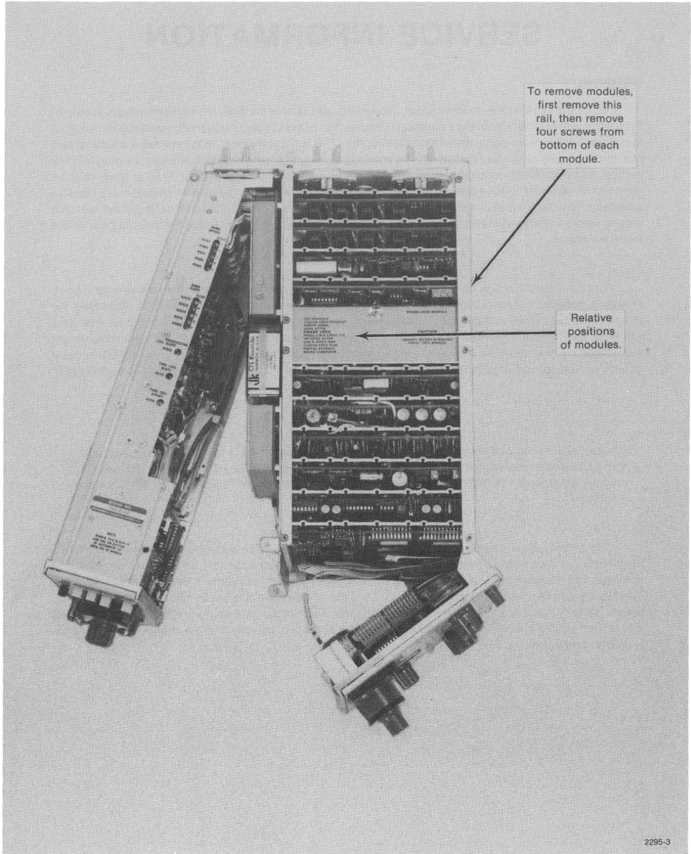
Figure 3-1. 7L18 Extended for servicing.
