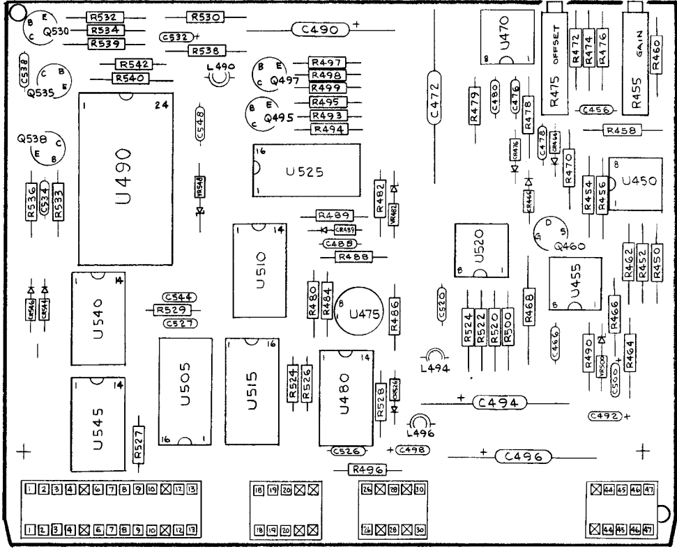
7L18 H-5010-01 A450 CENTER FREQUENCY DVM
