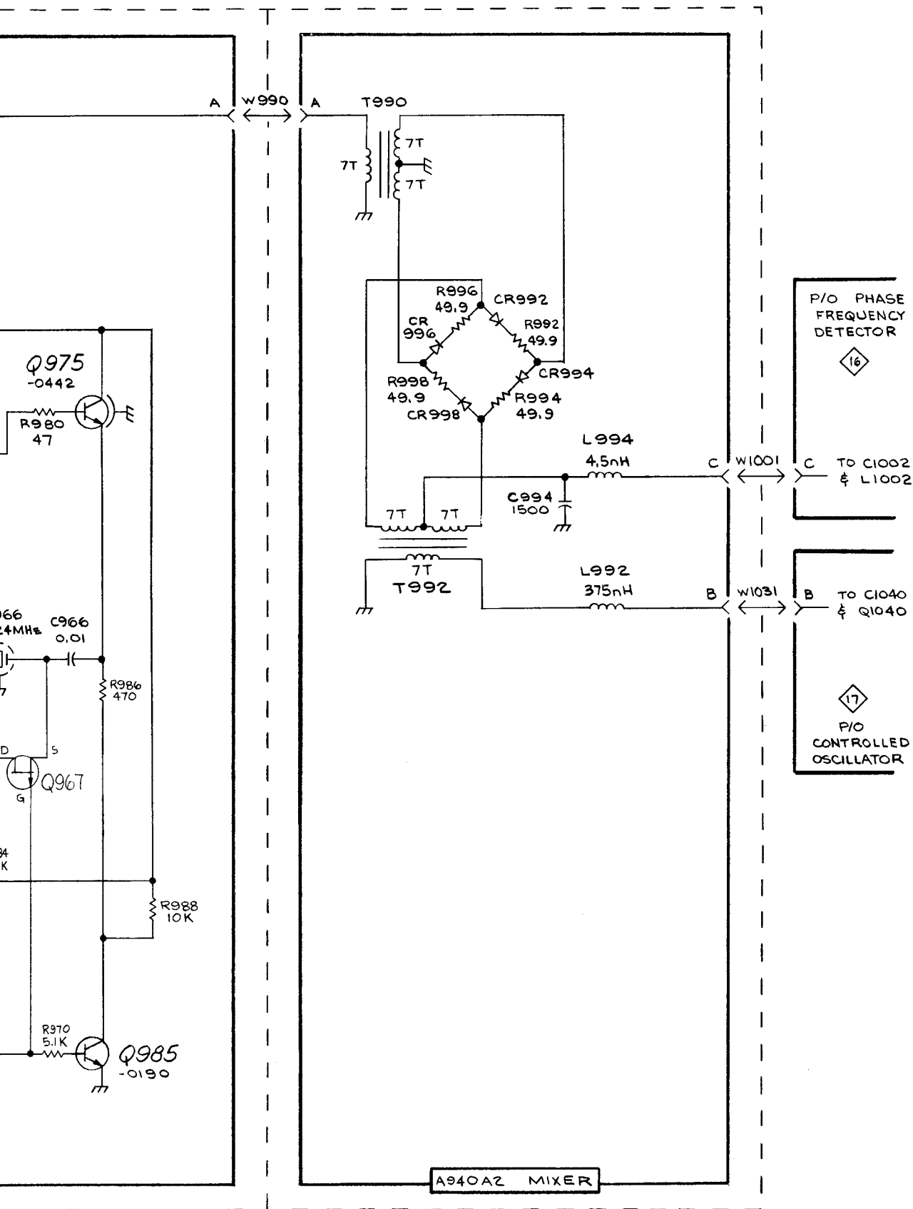
REFERENCE OSCILLATOR & MIXER 15
