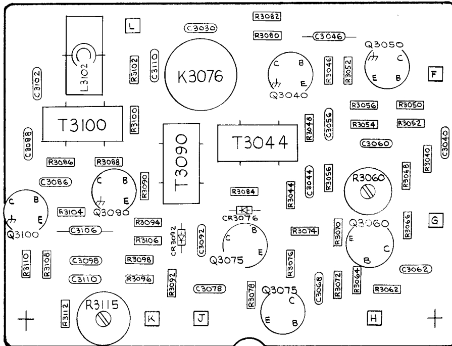
7L18 A3000A2 VARIABLE RESOLUTION PRE-AMPLIFIER H-5205-00
