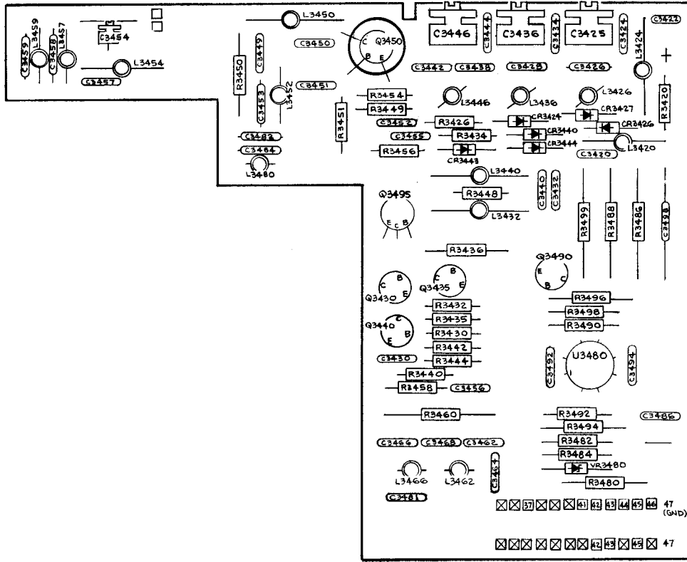
7L18 H-5012-02 A3420 VARIABLE RESOLUTION NOISE FILTER
