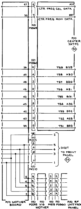
CENTER FREQUENCY READOUT
