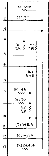
LOG AMPL RESISTOR ASSEMBLY TYPICAL OF: R578, R592, R622, R652, R672, R692 & R702
