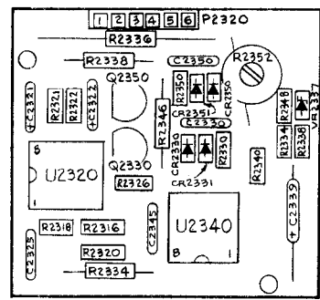
H-5026-01 7L18 A2316 REFERENCE VOLTAGES
