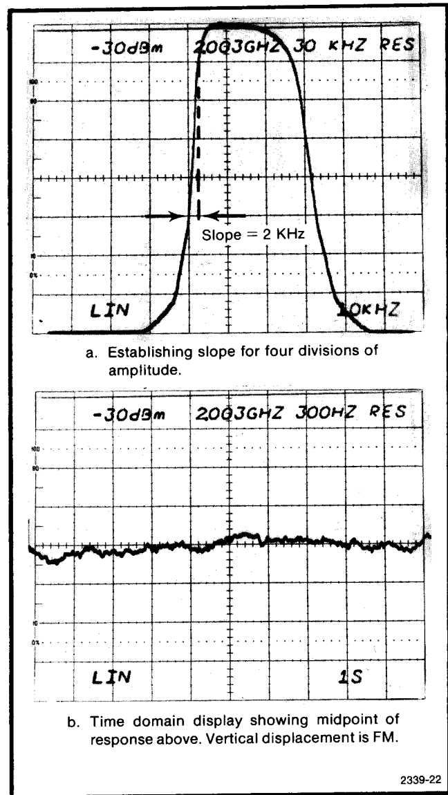
Fig. 4-8. Measuring Incidental FM.
