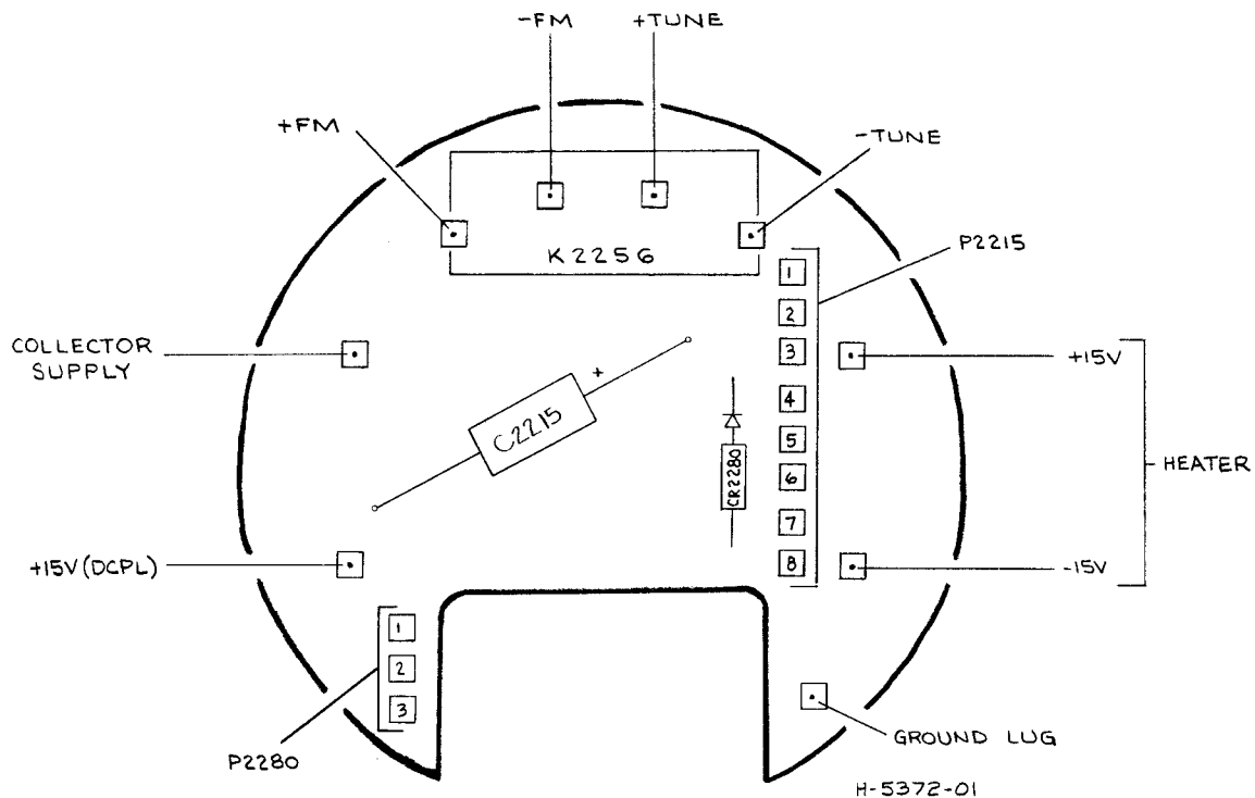
7L18 A60A1 1ST LO BOARD
