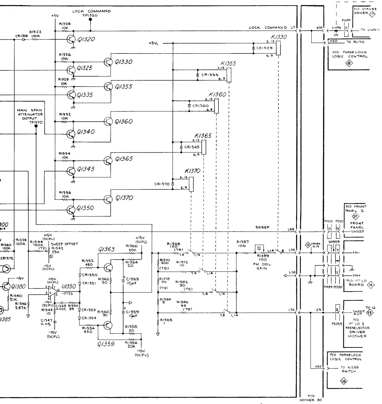
SPAN ATTENUATOR (2)
