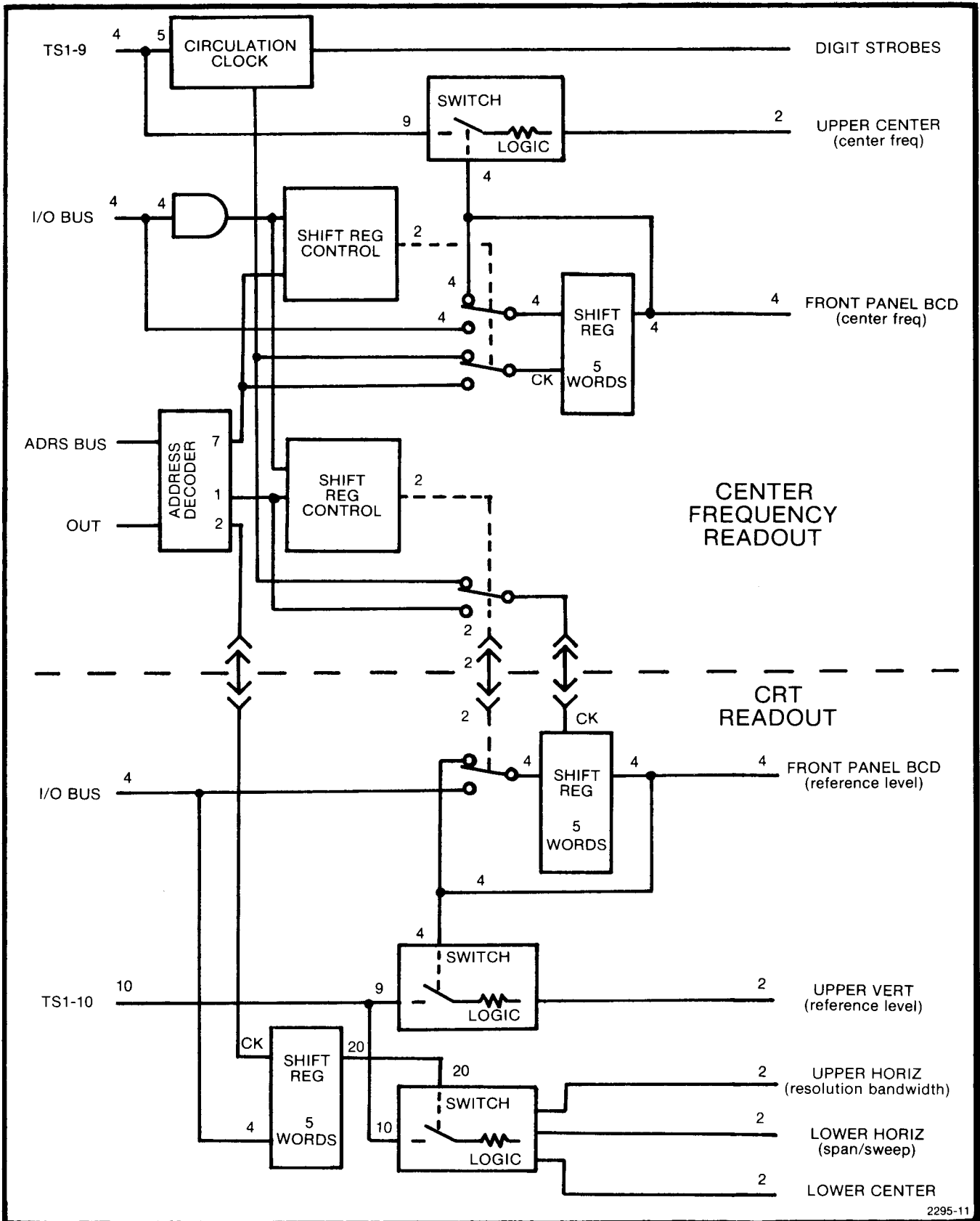
Figure 2-7. Readout block diagram.
