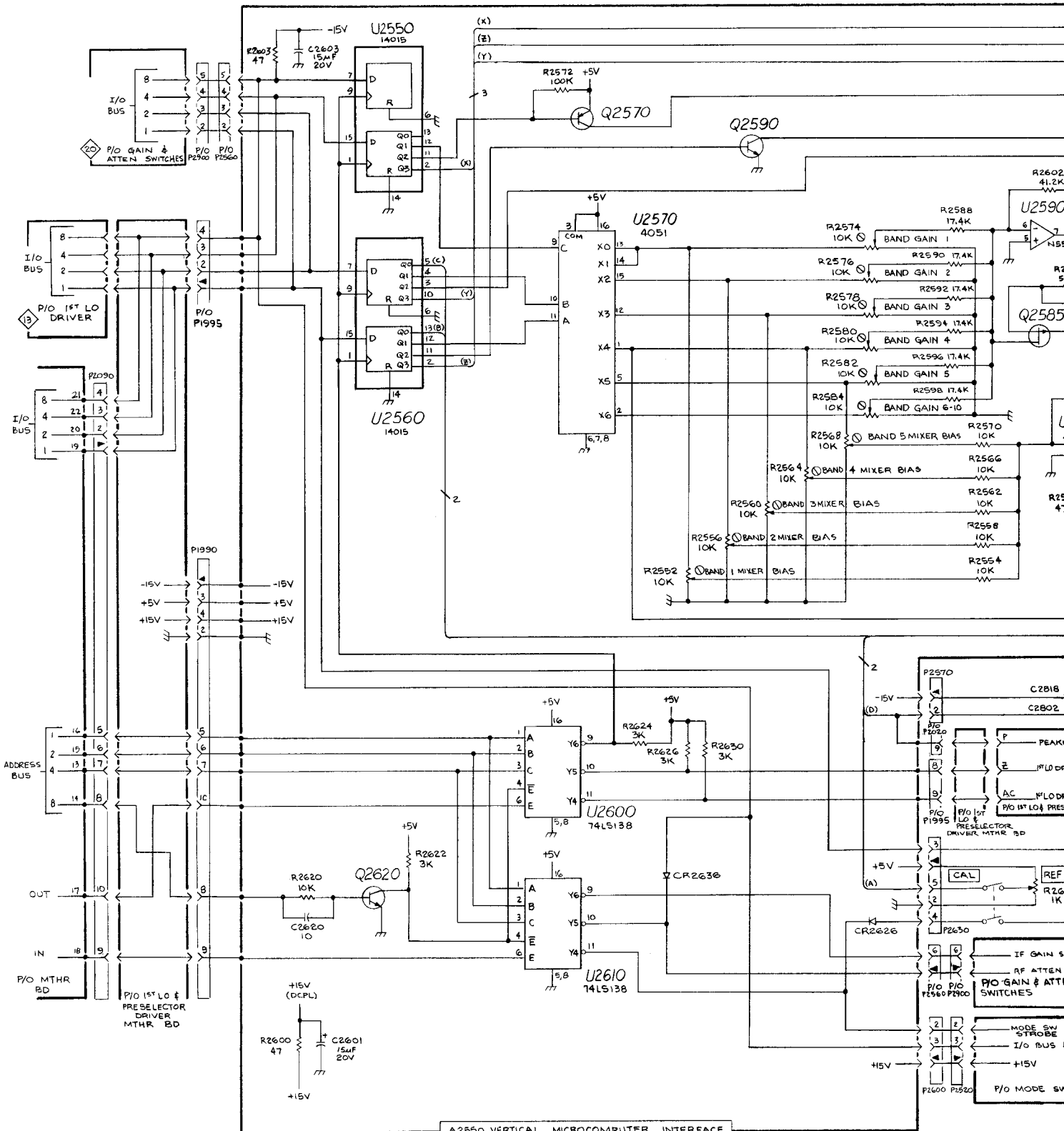
A2550 VERTICAL MICROCOMPUTER INTERFACE
