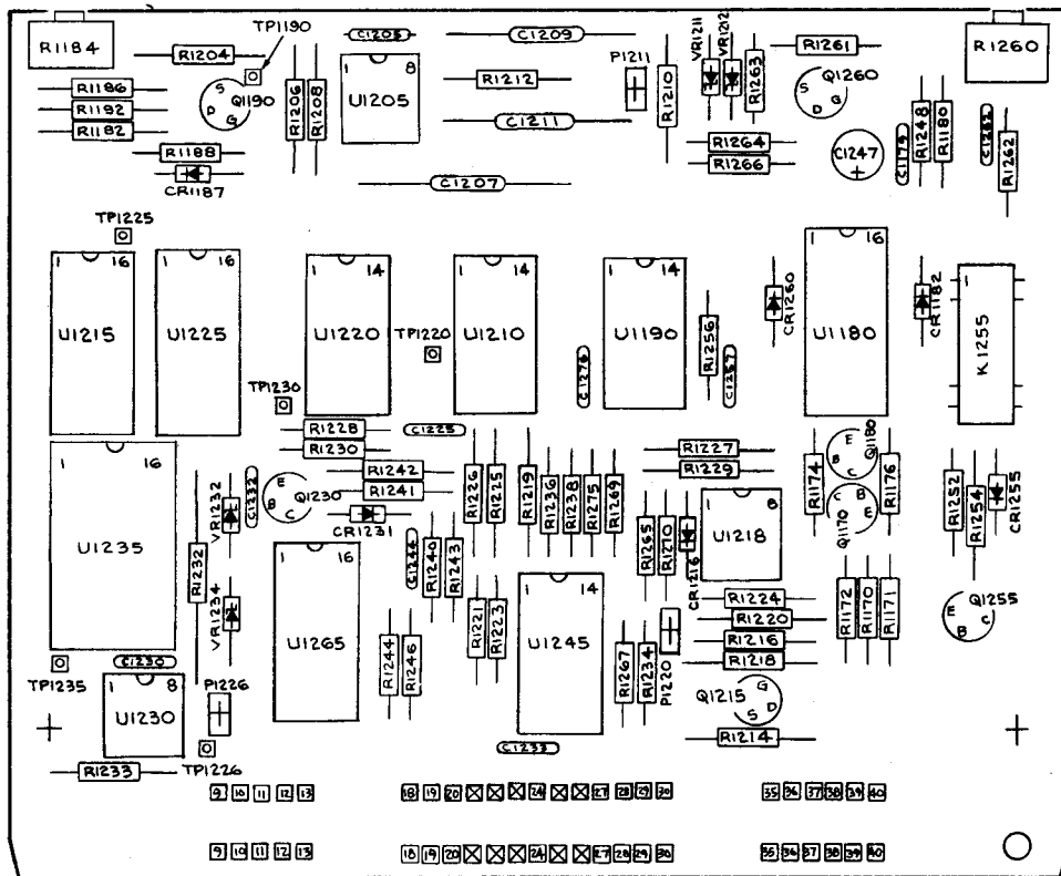
7L18 H-5011-01 A1170 PHASELOCK LOGIC CONTROL
