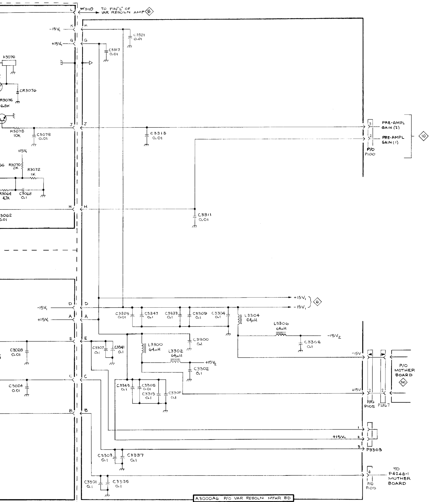
A3000 VARIABLE RESOLUTION 5
