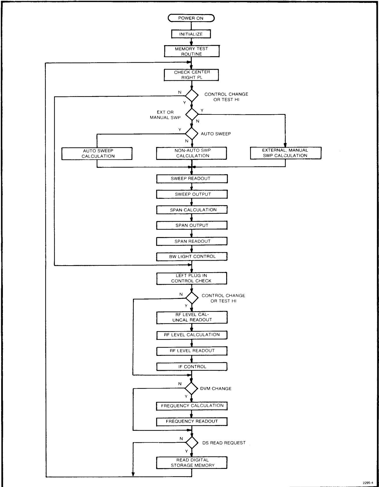
Figure 2-6. Control Program Simplified diagram.
