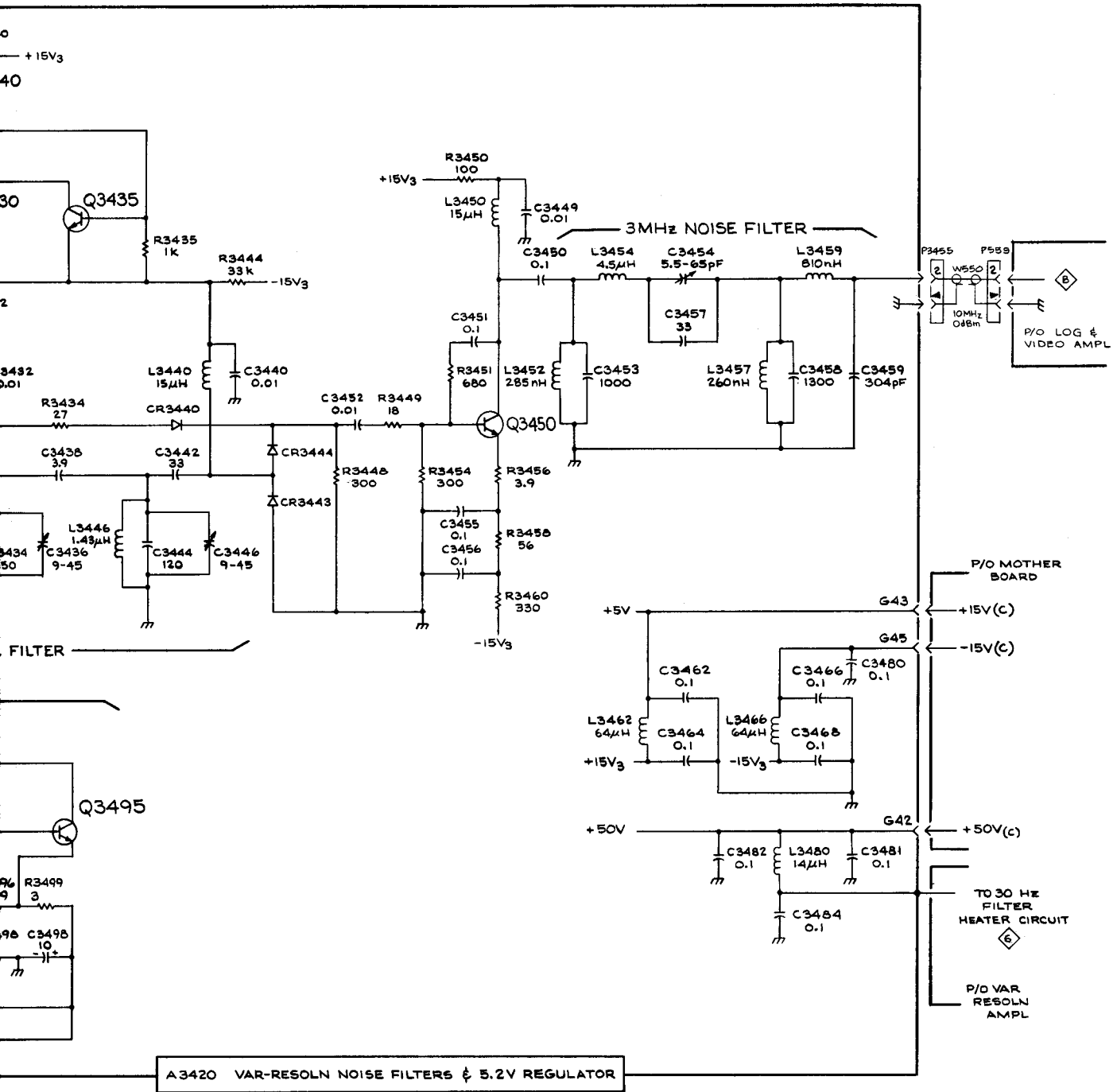
VAR-RESOLN NOISE FILTERS & 5.2V REGULATOR
