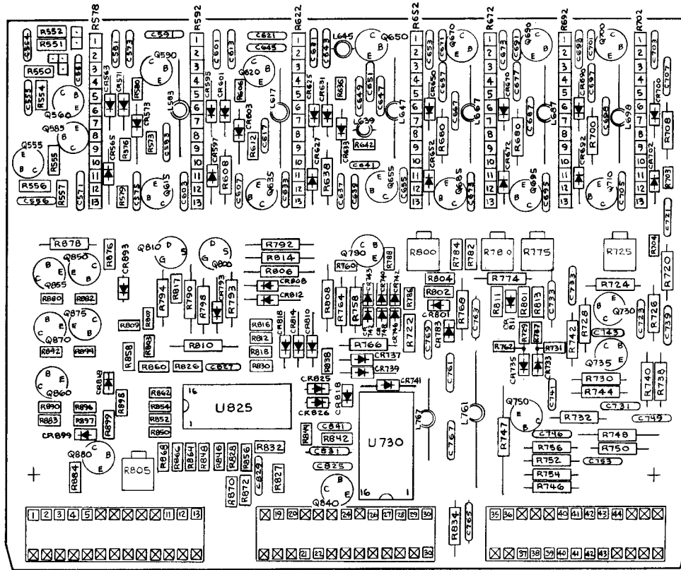
7L18 H-5009-00 A550 LOG & VIDEO AMPLIFIER
