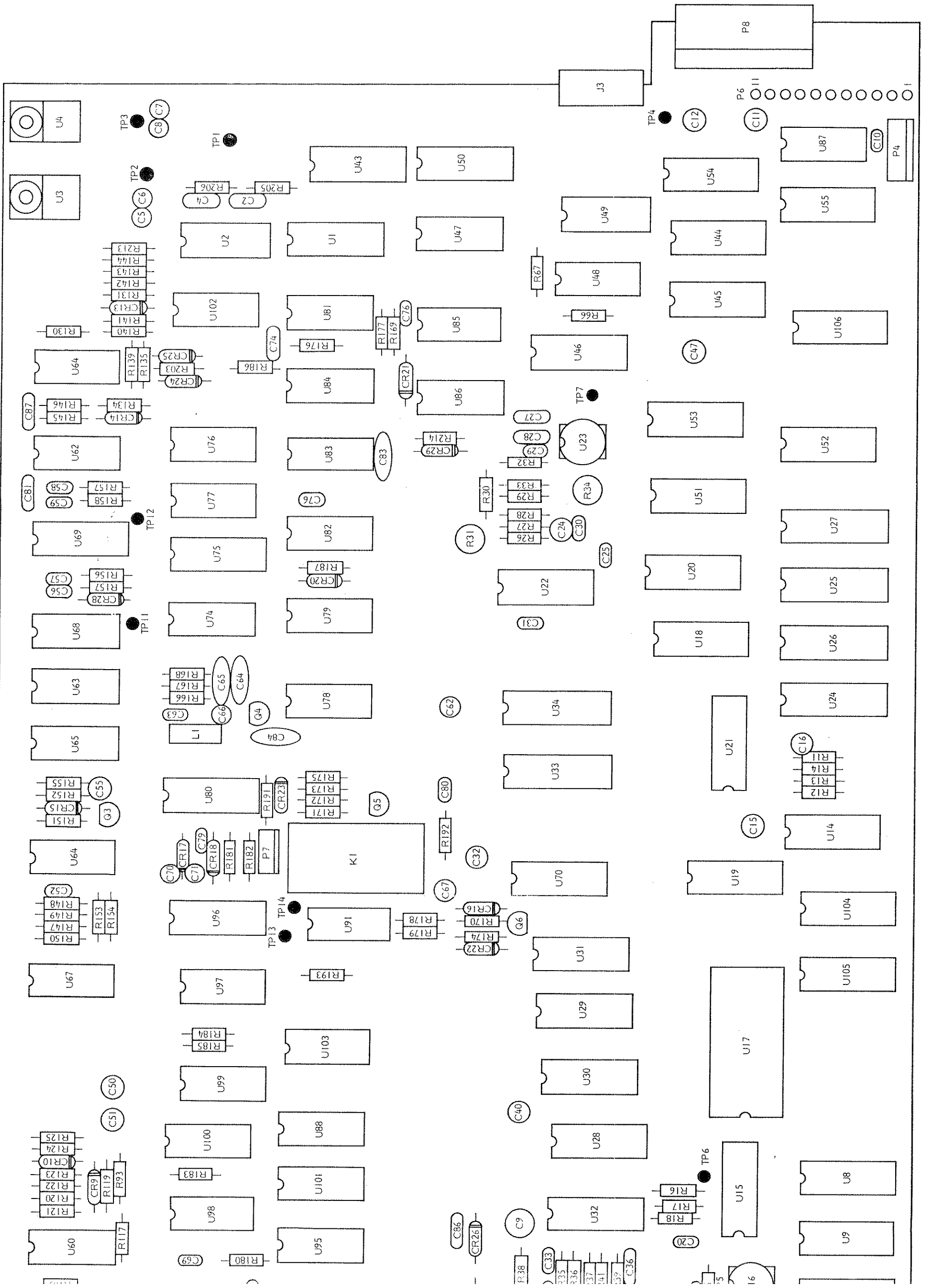
Fig. 5-15 A2 (Digital) board
