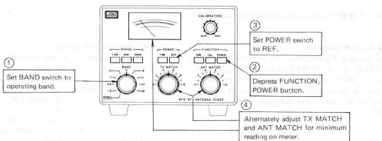
Figure 3.3 Matching Network Adjustment
