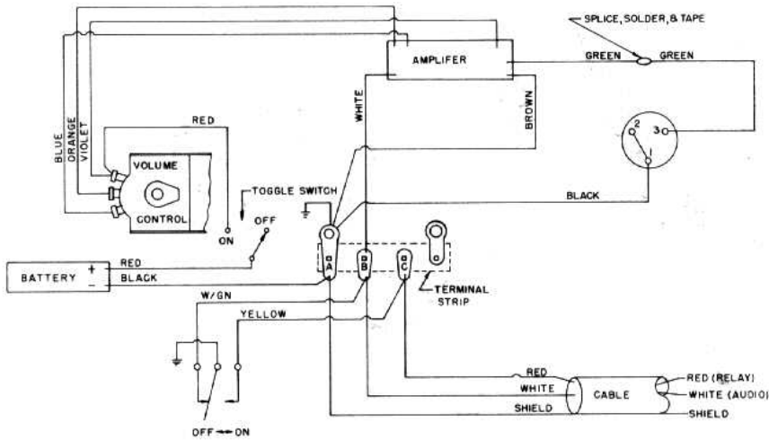
TG-KIT WIRING DIAGRAM REV 1 FIG 3
