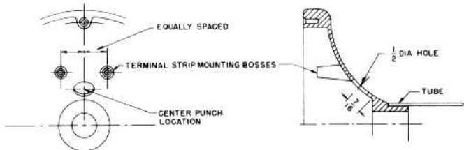
CROSS SECTION VIEW THROUGH PORTION OF BASE SHOWING LOCATION OF 1/2" DIA. HOLE FIG 1
