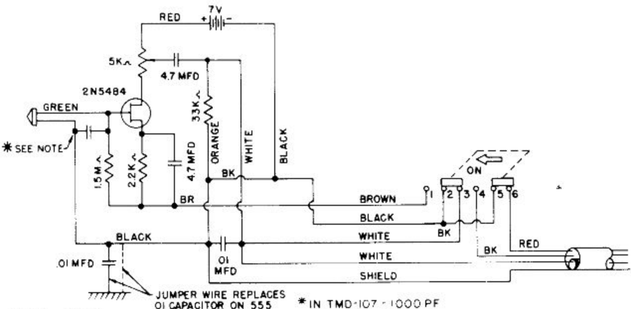
TMD-107-E (ELECTRONIC), DIO4-M (ELECTRONIC) & 555 TRUCKER (ELECTRONIC) SCHEMATIC
