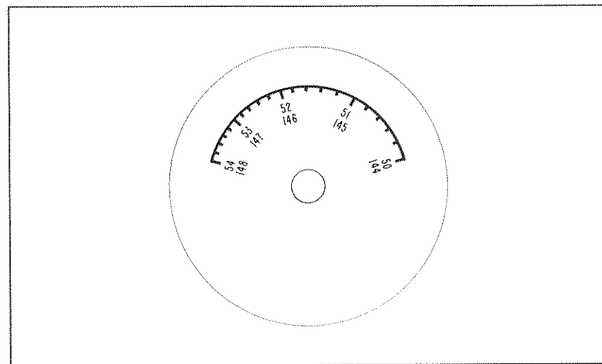
Figure 5. Dial Scale Calibrations.
