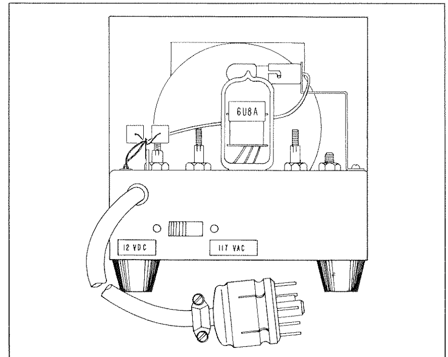
Figure 2. Rear View of VFO.
