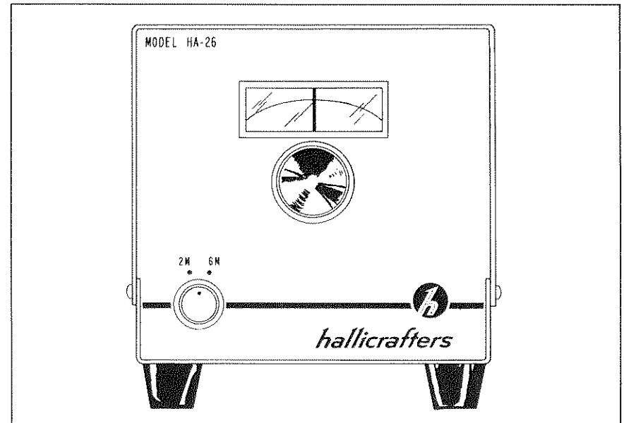
Figure 4. Front Panel View of VFO.
