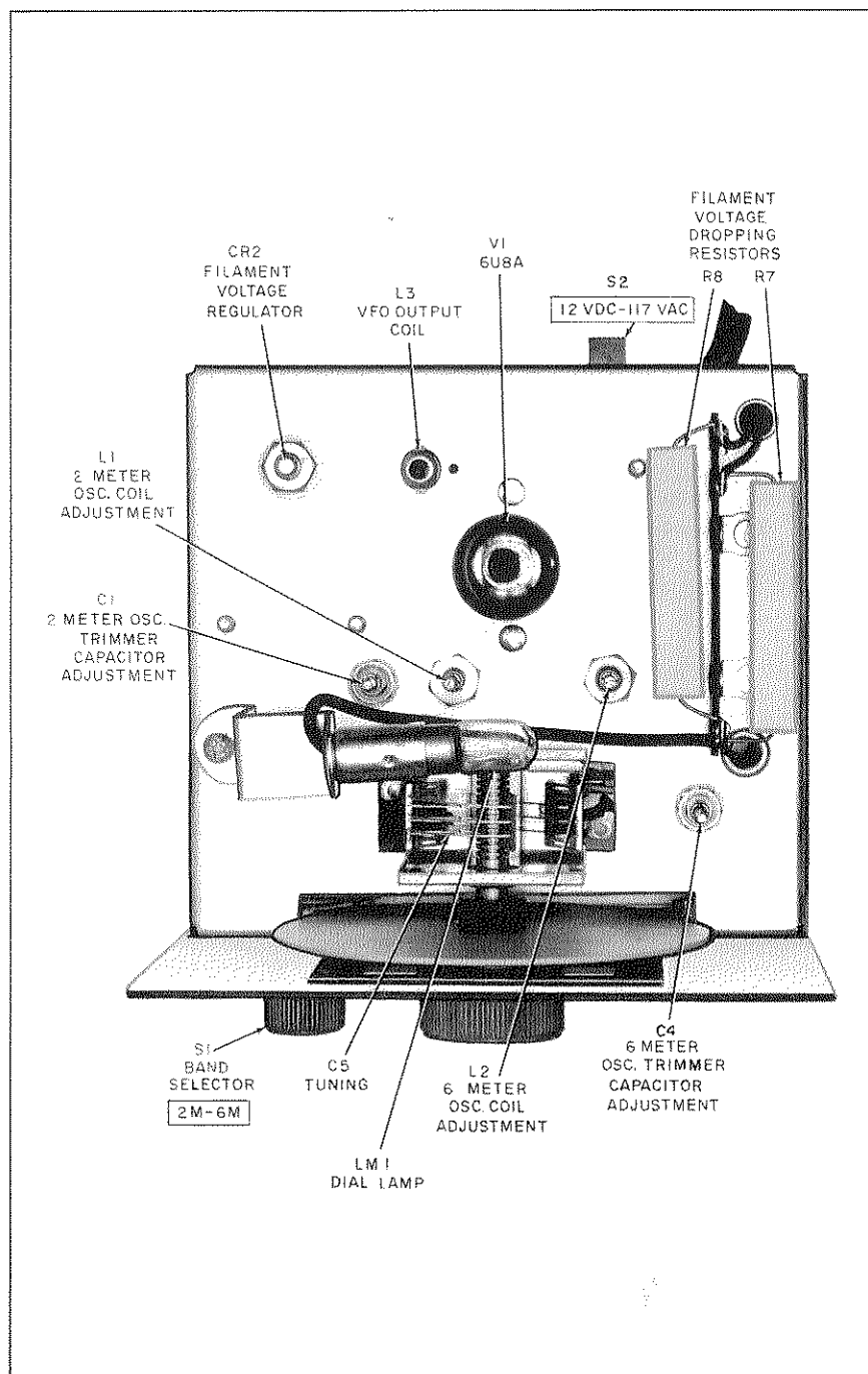
Figure 6. Top View of VFO Chassis.
