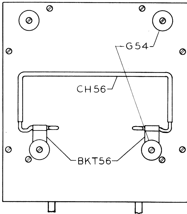
CABINET BOTTOM AND TILT STAND
