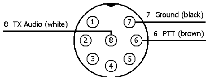
Female Connector (Wiring Side)
