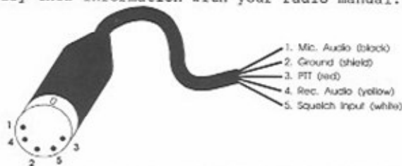
Fig. 3-2 Radio Connector Pin Diagram
