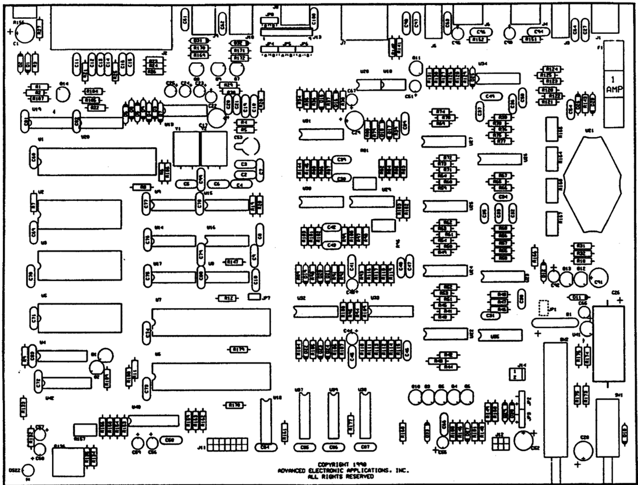
MAIN BOARD
