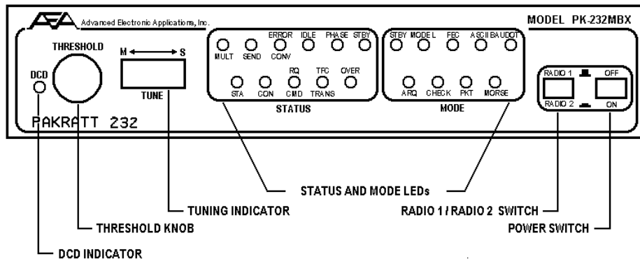
Figure 2-1 PK-232 Front Panel Controls and indicators
