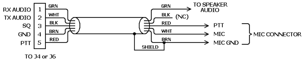
Figure 3-6 Radio-to-PK-232 Connections
