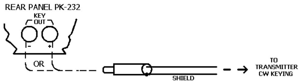
Figure 3-3 Direct CW Keying Cable diagram
