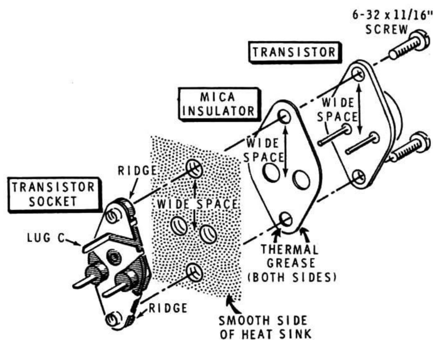
Detail 2-5A
