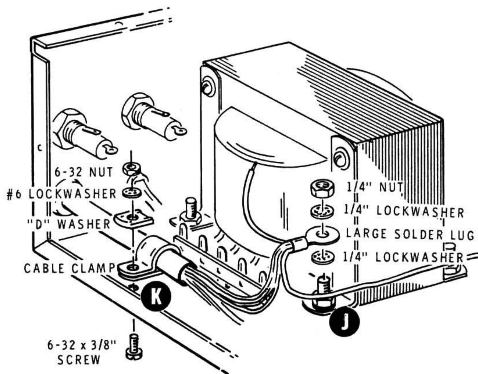
PICTORIAL 2-4
