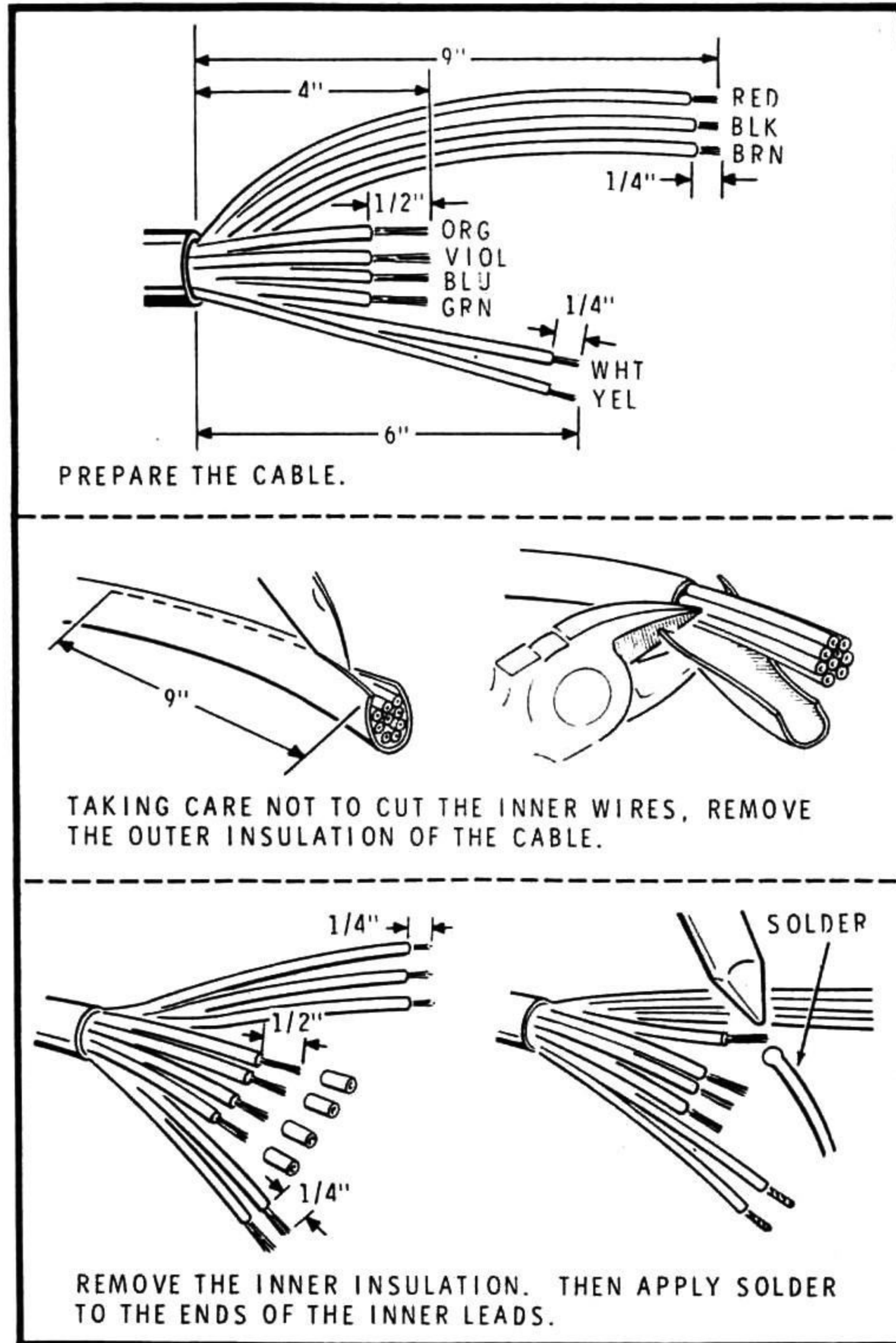
PICTORIAL 2-2
