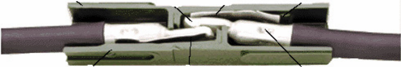
Internal view of two Powerpoles® connected. (Anderson Power drawings; www.andersonpower.com )
