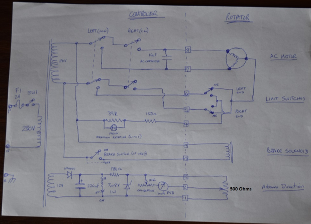
re-drawn circuit diagram with 230V to 110V + 12V transformer
