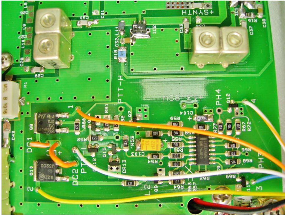
20. VR3, R21, NTC install and general wiring.
