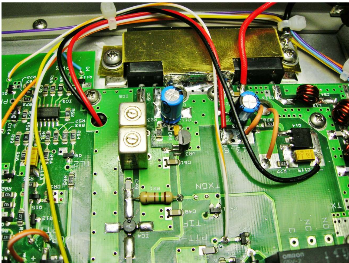
20. VR3, R21, NTC install and general wiring.
