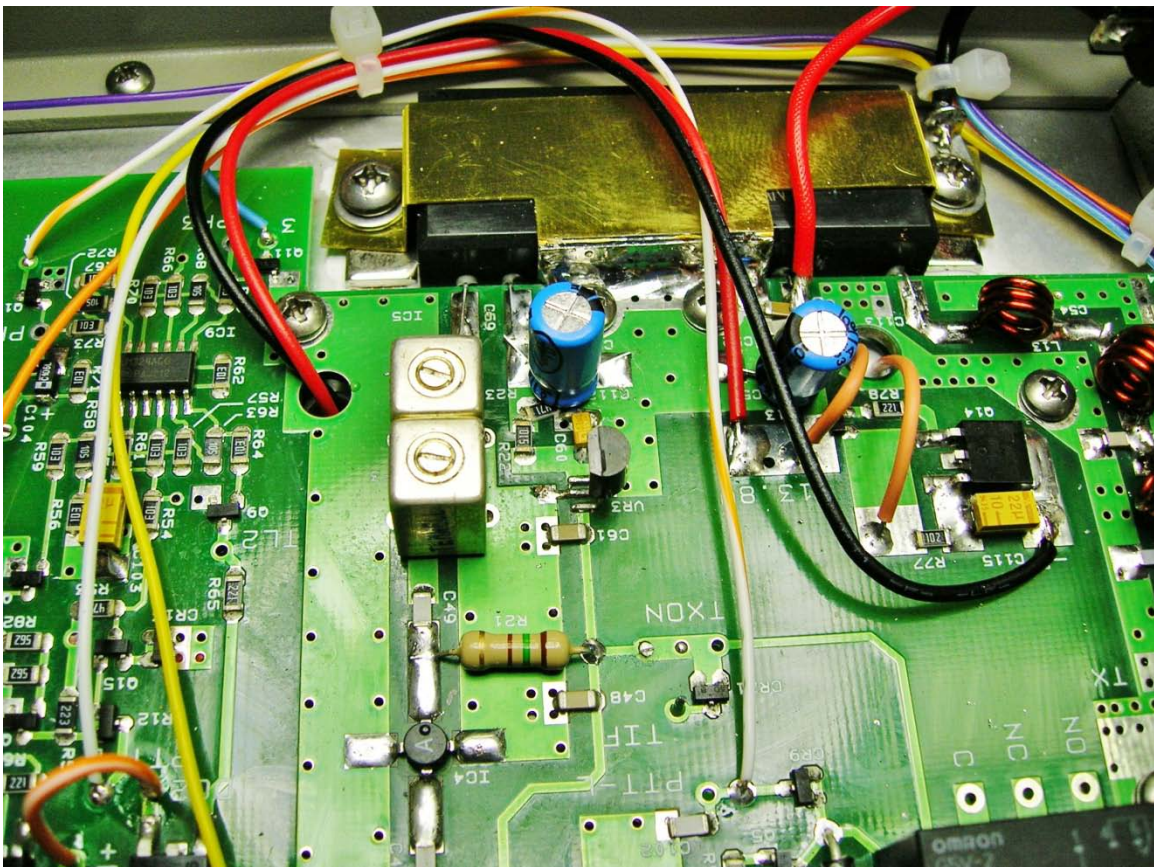
20. NTC install, Fan and other general wiring.
