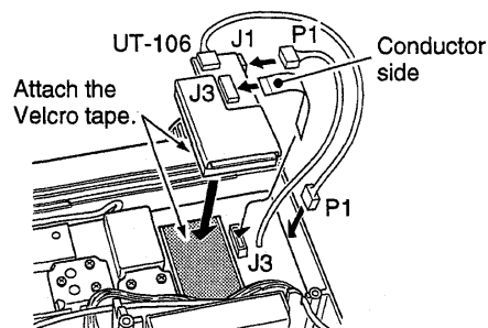
PLL unit
