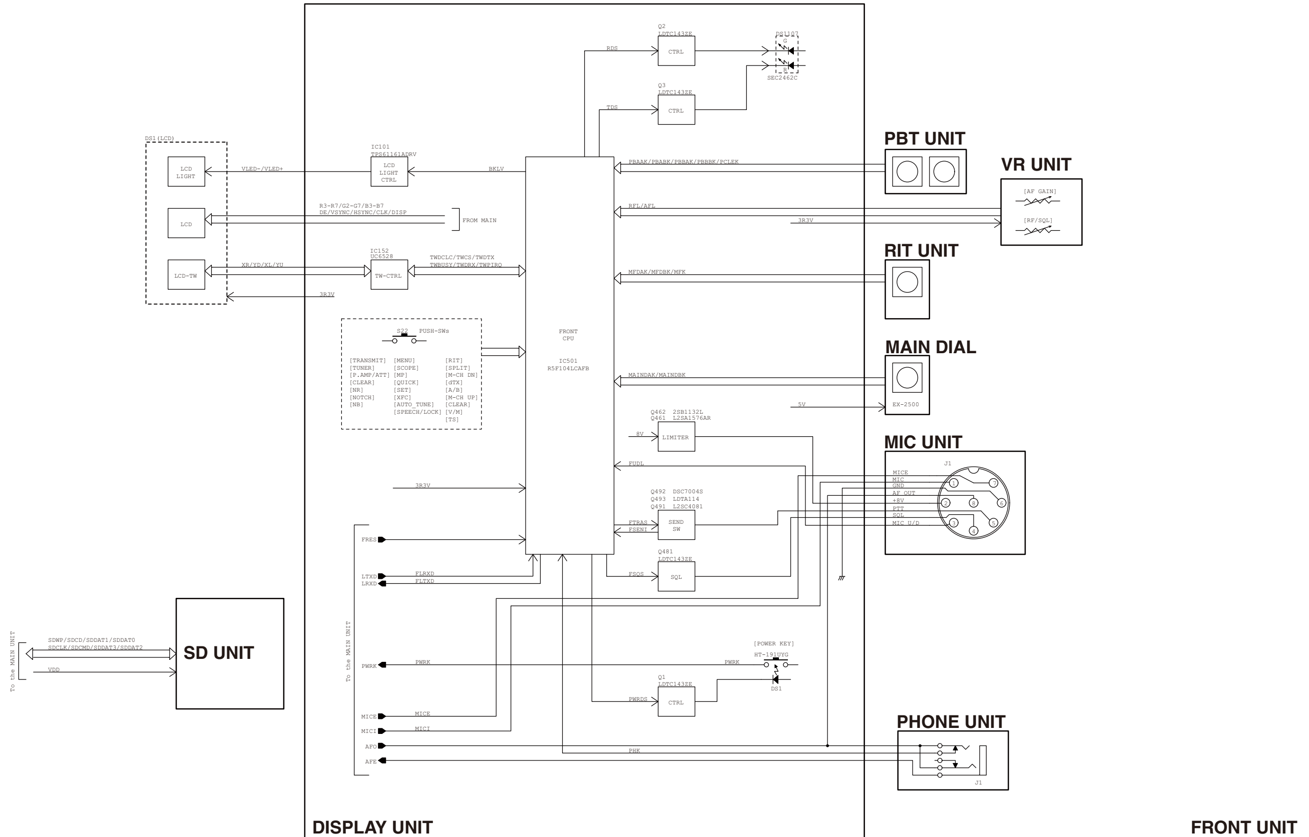
BLOCK DIAGRAM (BLOCK DIAGRAM-3)
