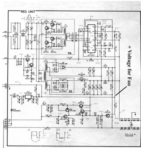
Power Supply Schematic
