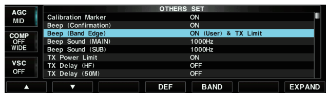
ON (User) & TX Limit is selected
