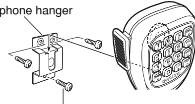
Microphone hanger screw (3 mm x 10 mm)
