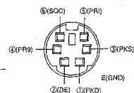
Pin assignment seen from direction B
