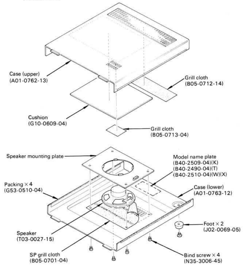
Fig. 12 Case disassembly
