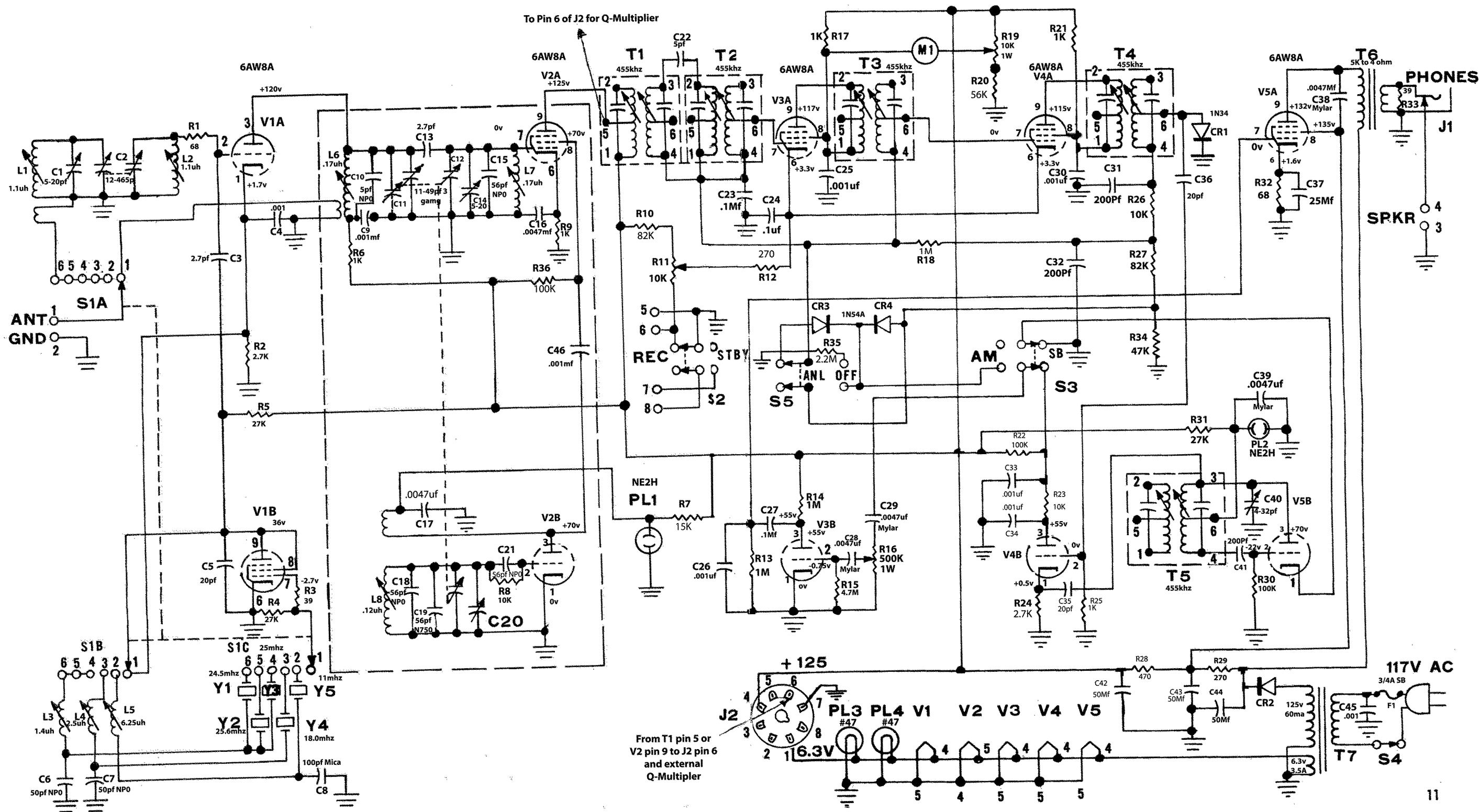
FIG. 5, CHEMATIC DIAGRAM
