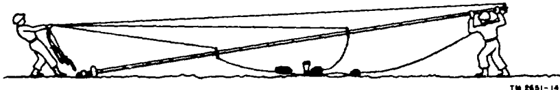
Figure 15. Raising mast.
