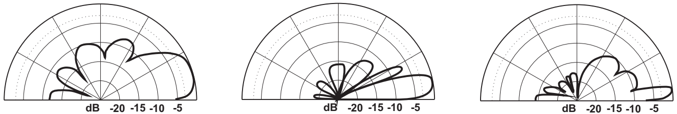
elevation radiation pattern
